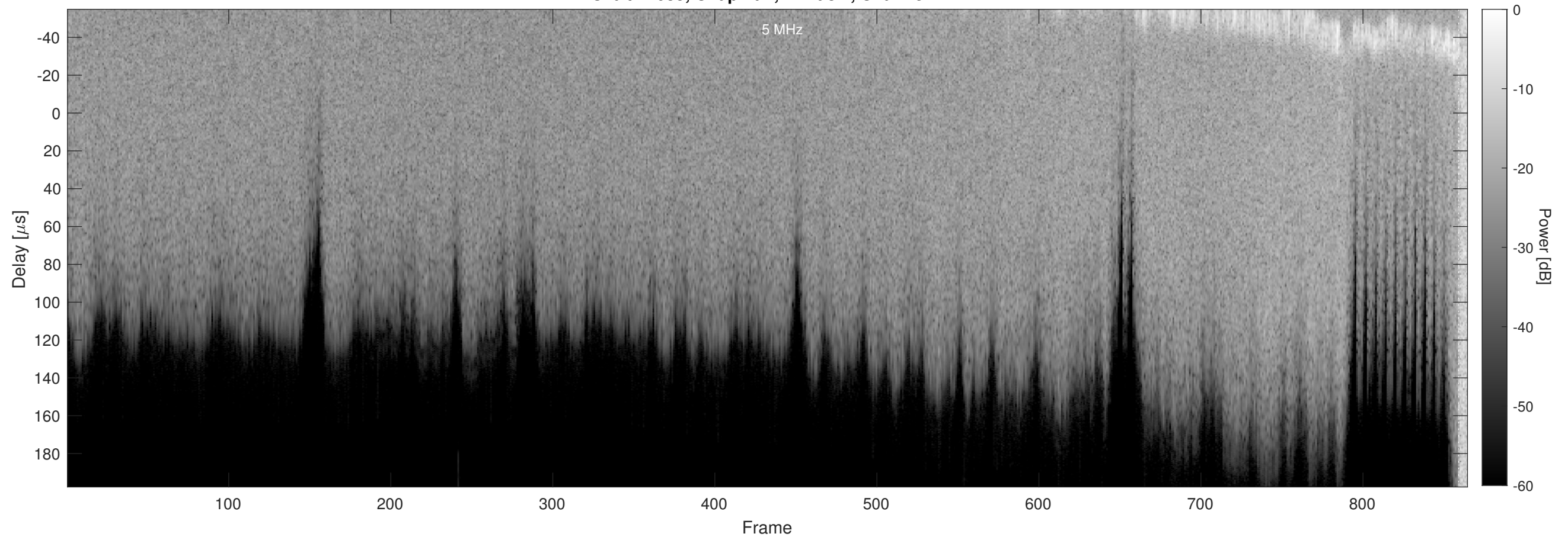
Orbit 21035, Chapman, Window, Channel 2
