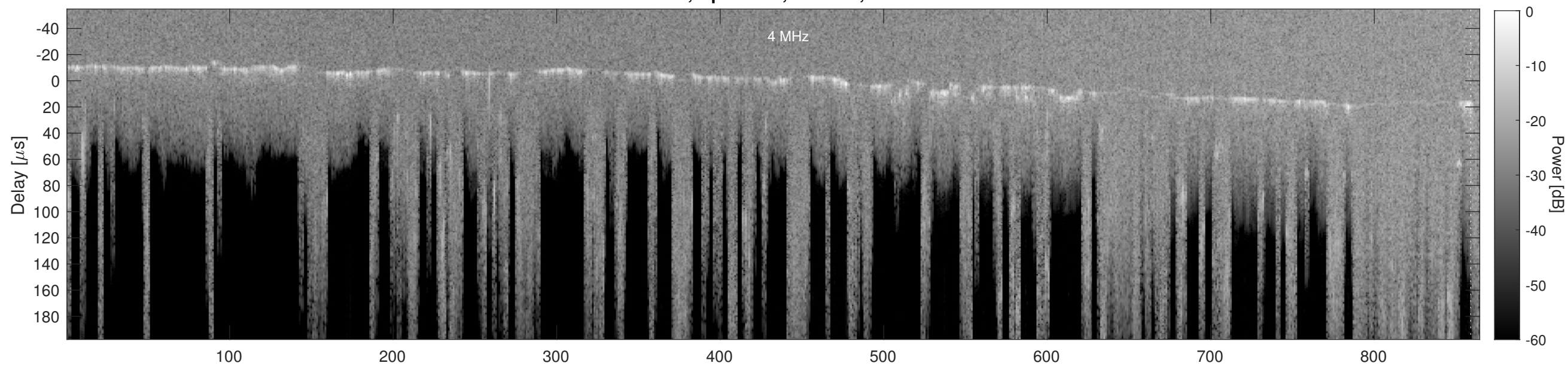
Orbit 21035, Cluttergram
