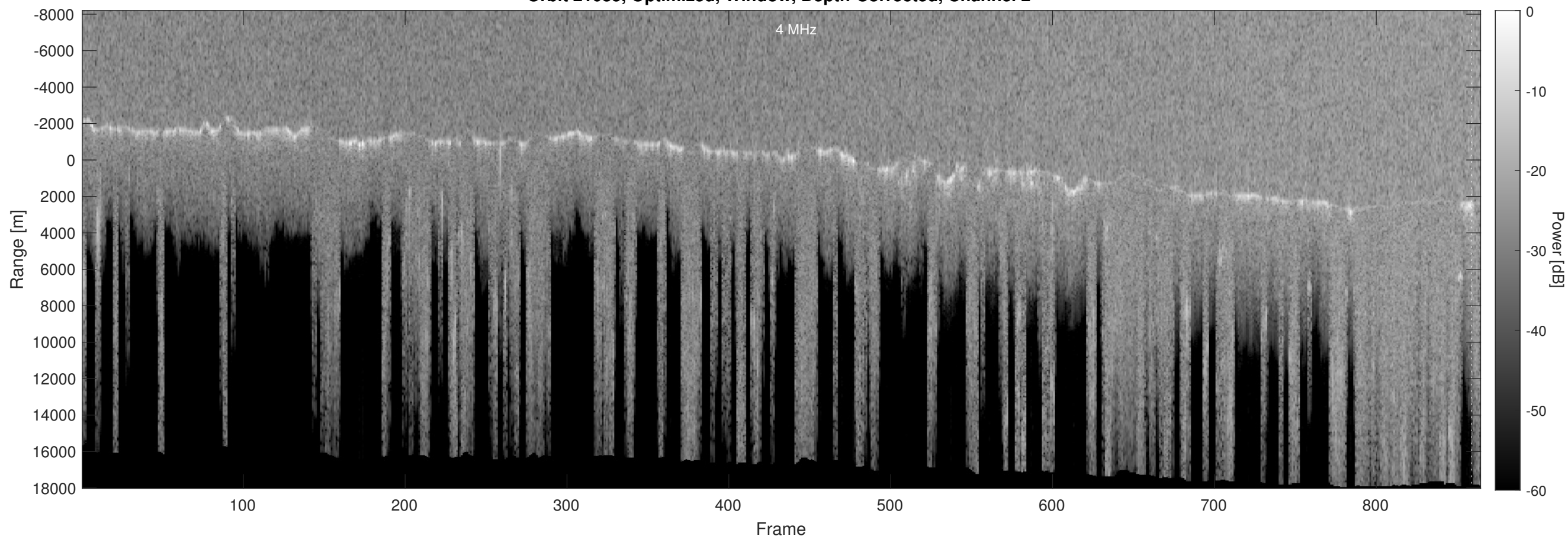
Orbit 21035, Optimized, Window, Depth-Corrected, Channel 2
