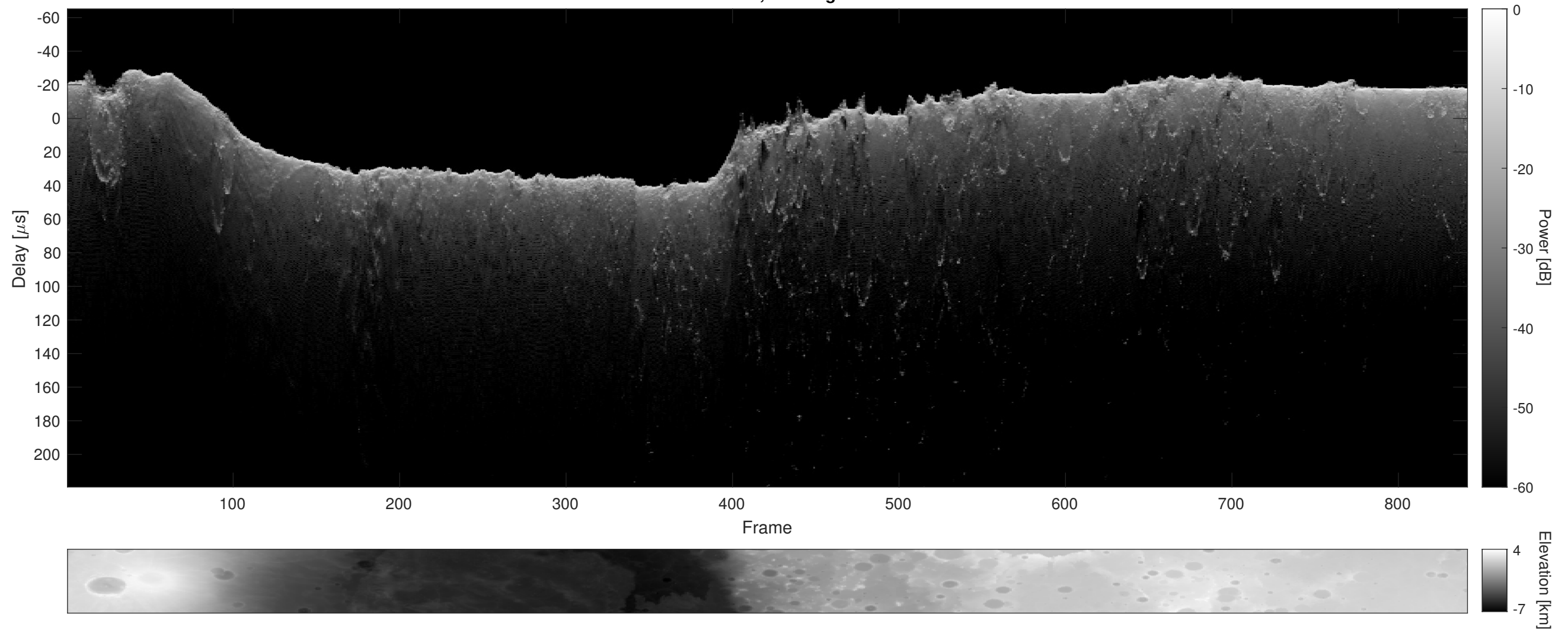
Orbit 21038, Cluttergram
