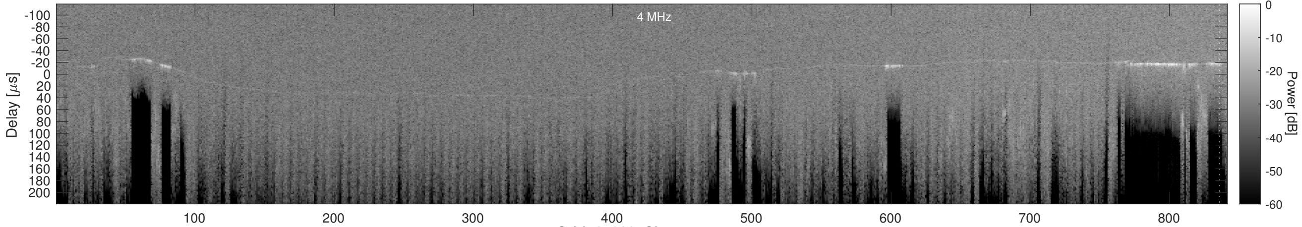
Orbit 21038, Cluttergram
