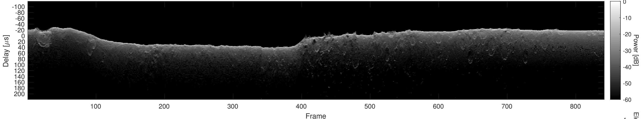
Orbit 21038, Cluttergram
