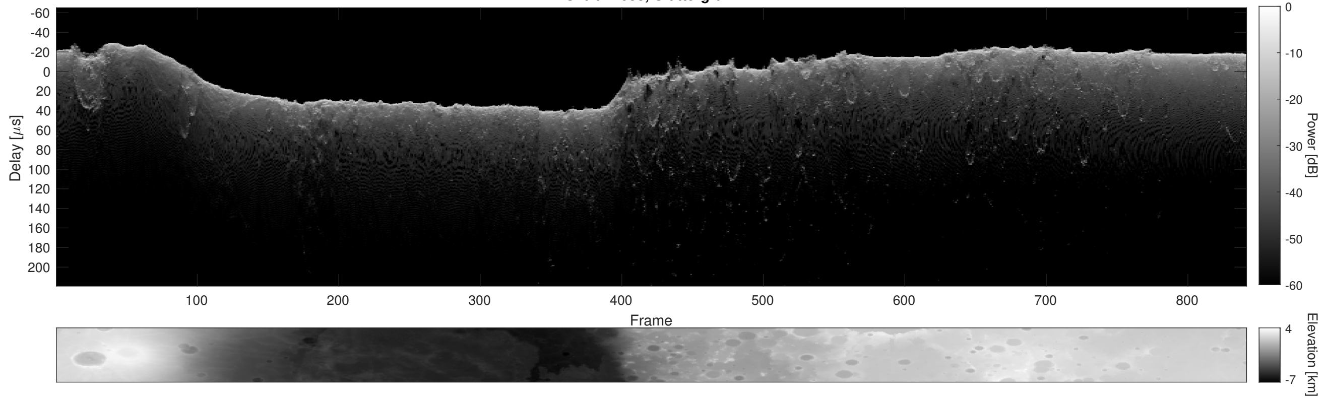
Orbit 21038, Cluttergram
