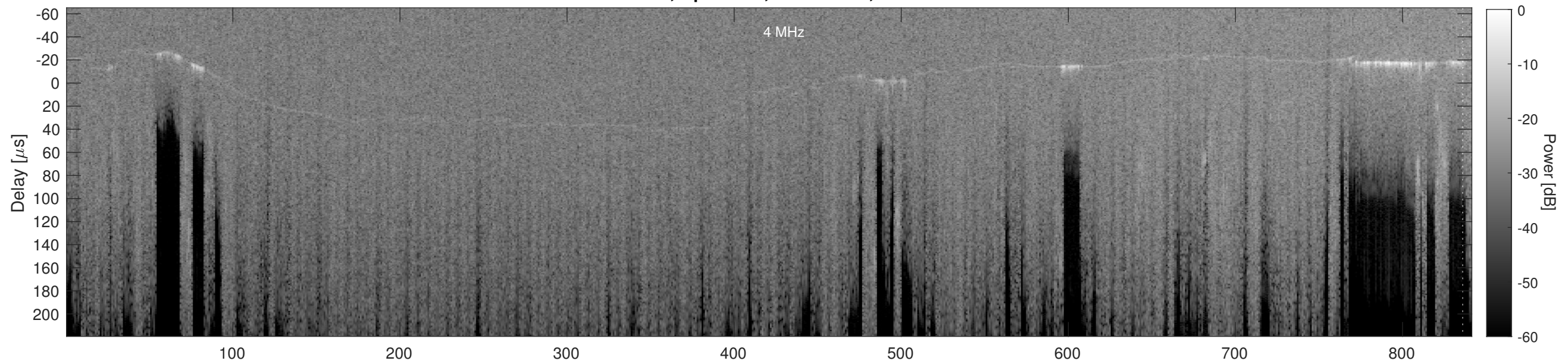
Orbit 21038, Cluttergram
