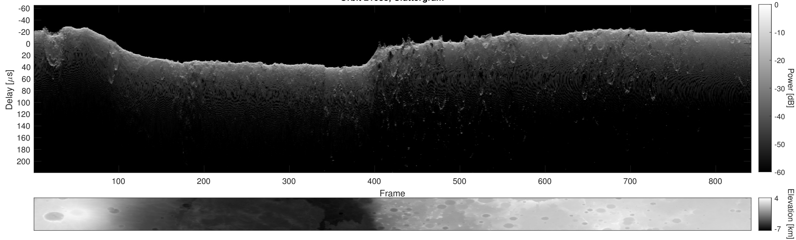
Orbit 21038, Cluttergram
