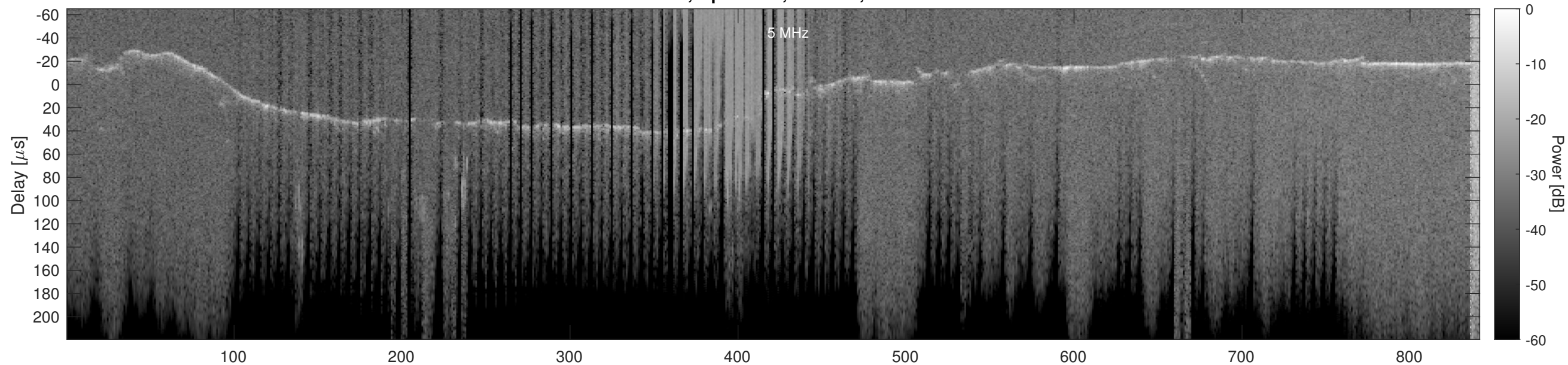
Orbit 21038, Optimized, Window, Channel 2
