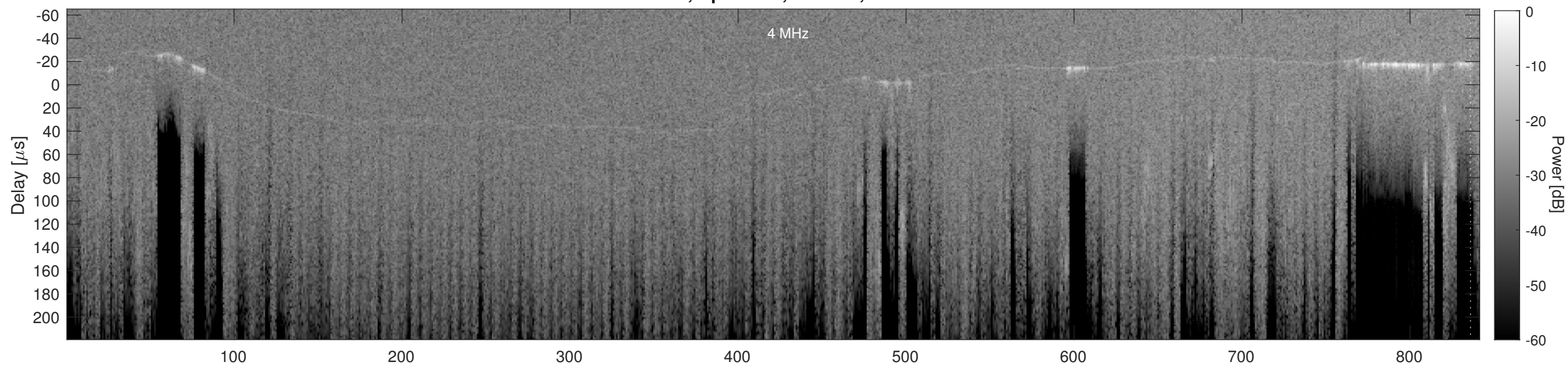
Orbit 21038, Cluttergram
