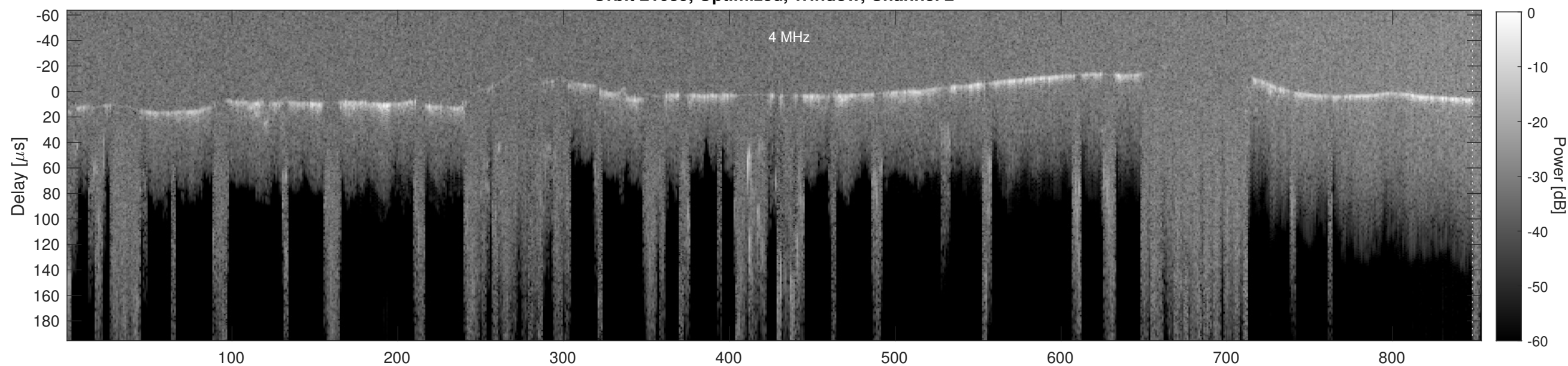
Orbit 21039, Cluttergram
