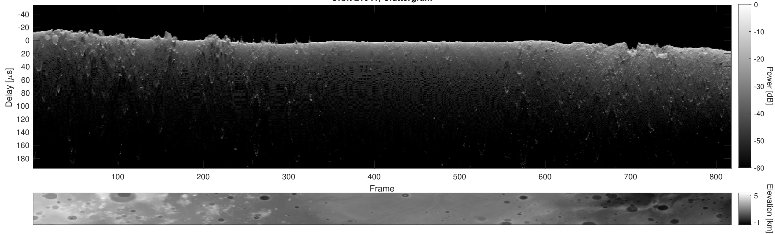
Orbit 21041, Cluttergram
