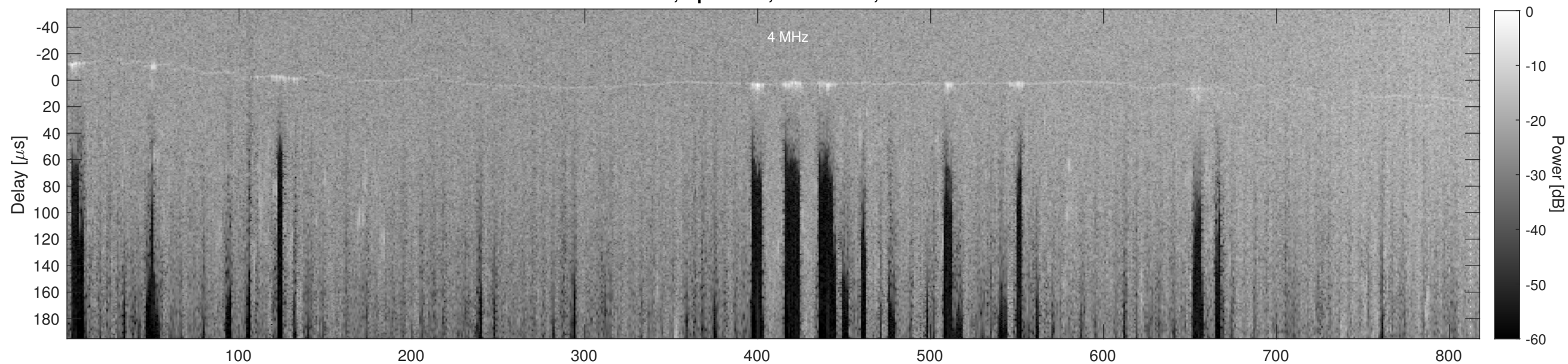
Orbit 21041, Cluttergram
