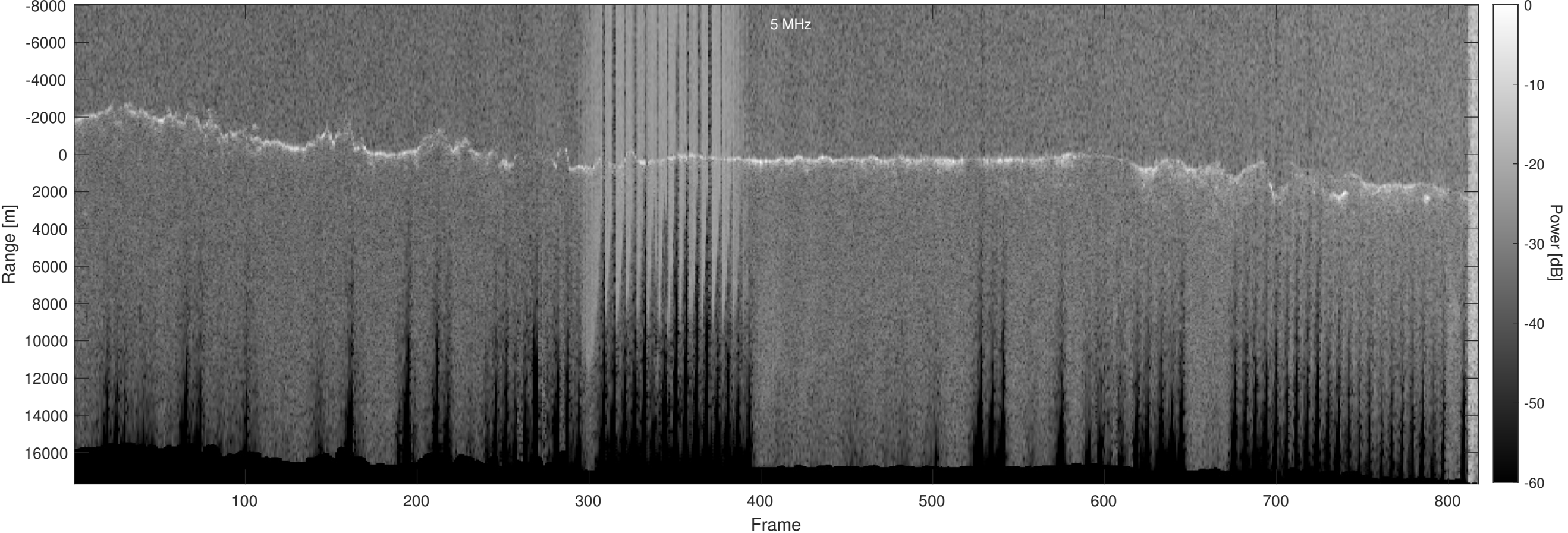
Orbit 21041, Optimized, Window, Depth-Corrected, Channel 2
