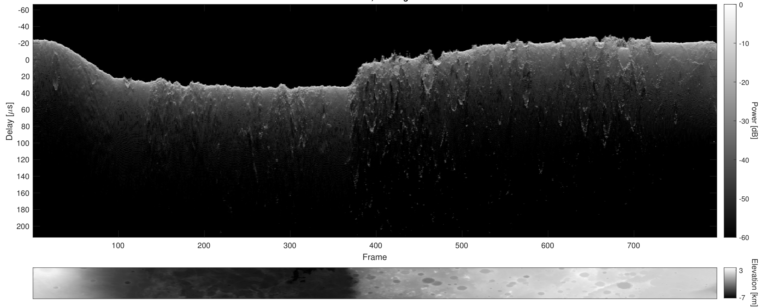
Orbit 21045, Cluttergram
