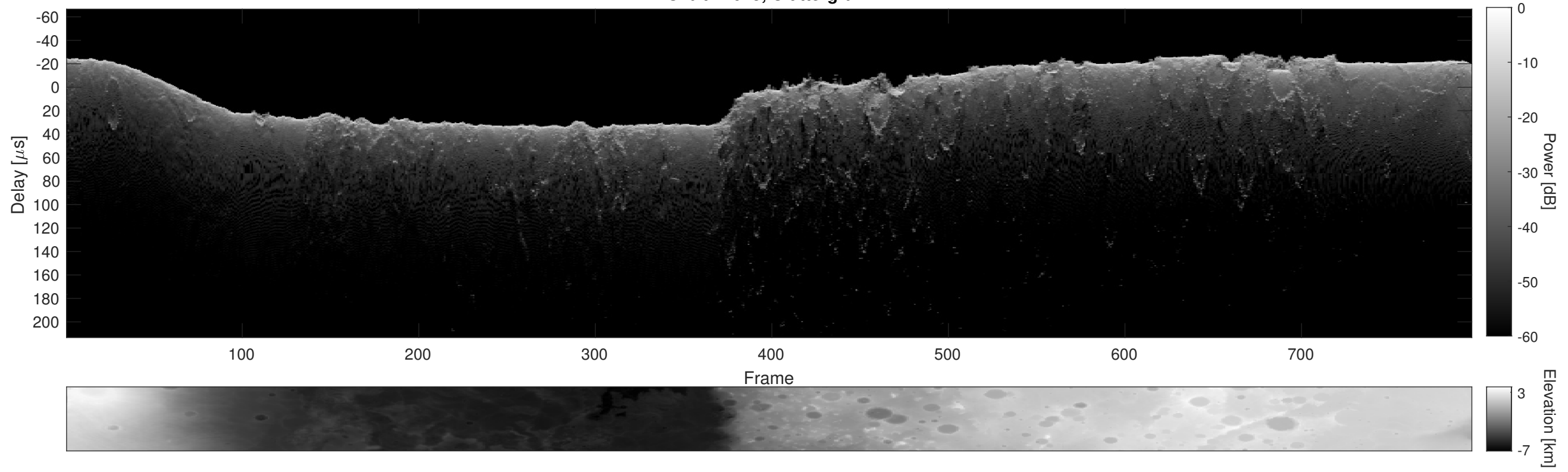
Orbit 21045, Cluttergram
