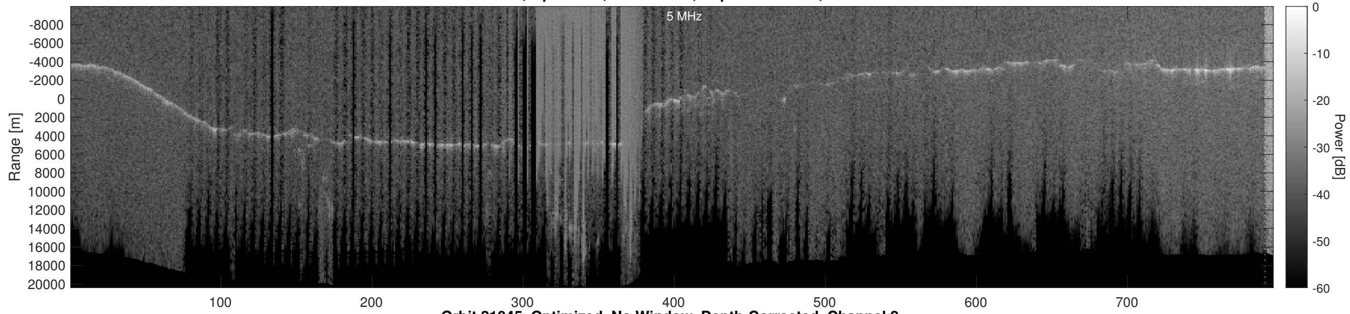
Orbit 21045, Optimized, No Window, Depth-Corrected, Channel 2
