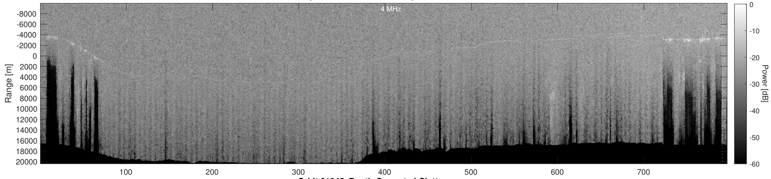
Orbit 21045, Depth-Corrected Cluttergram
