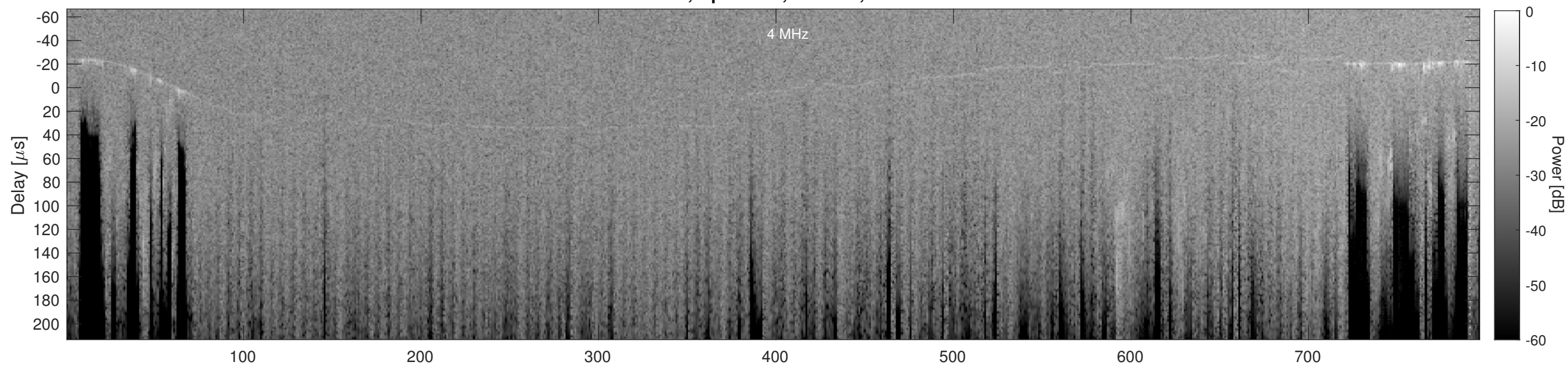
Orbit 21045, Cluttergram
