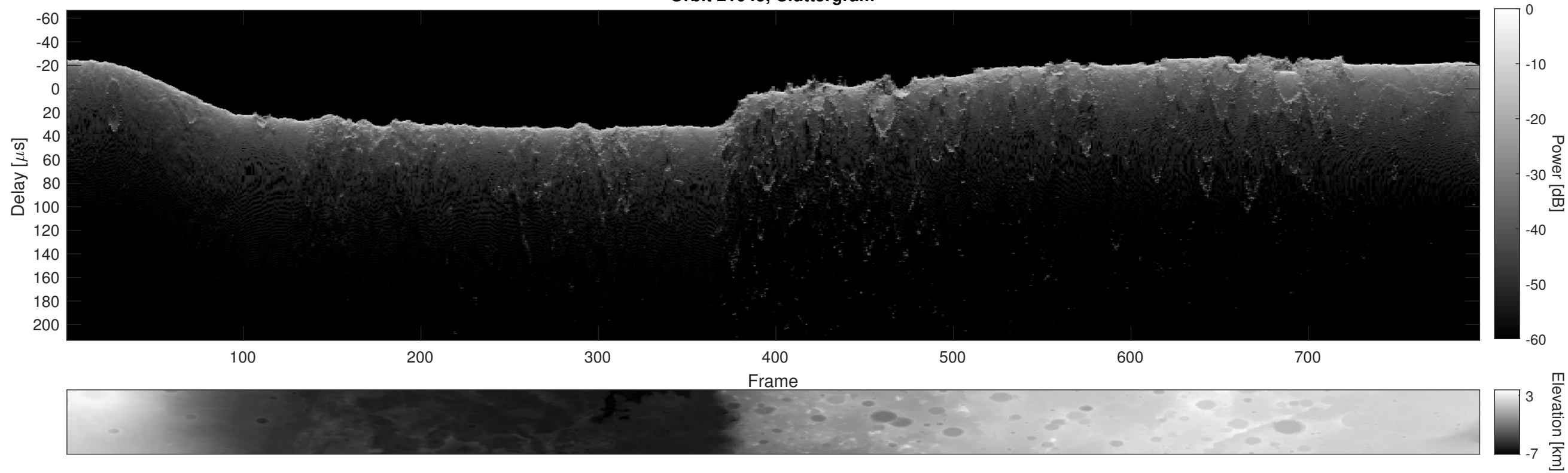
Orbit 21045, Cluttergram
