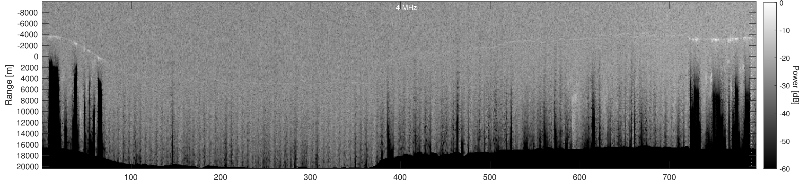
Orbit 21045, Depth-Corrected Cluttergram
