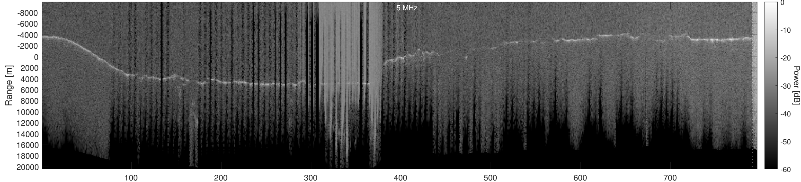
Orbit 21045, Optimized, Window, Depth-Corrected, Channel 2
