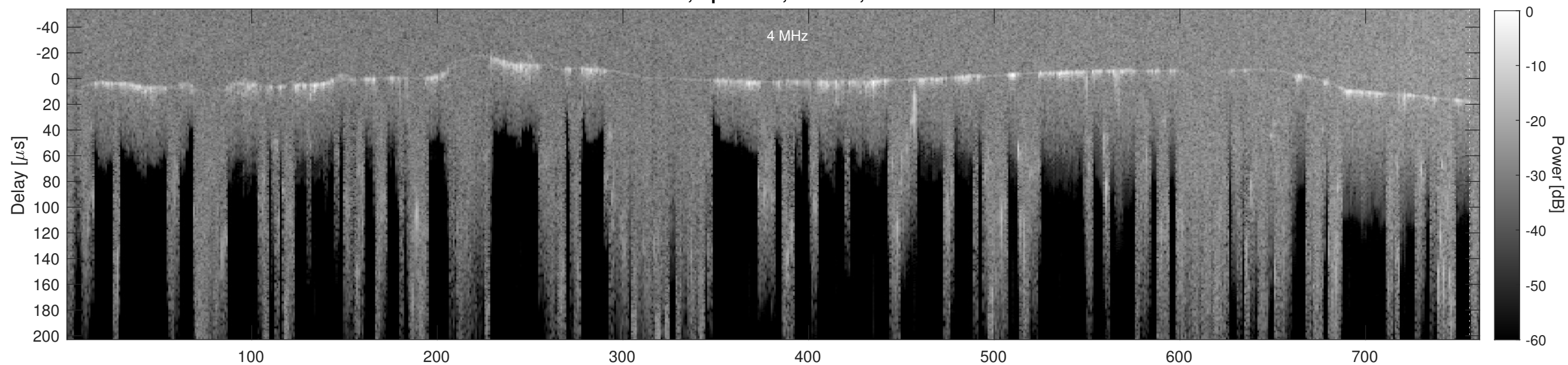
Orbit 21050, Cluttergram
