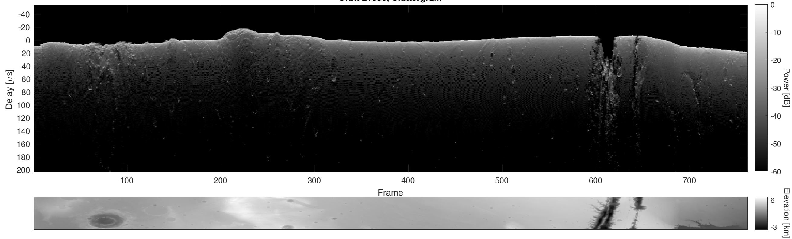
Orbit 21050, Cluttergram
