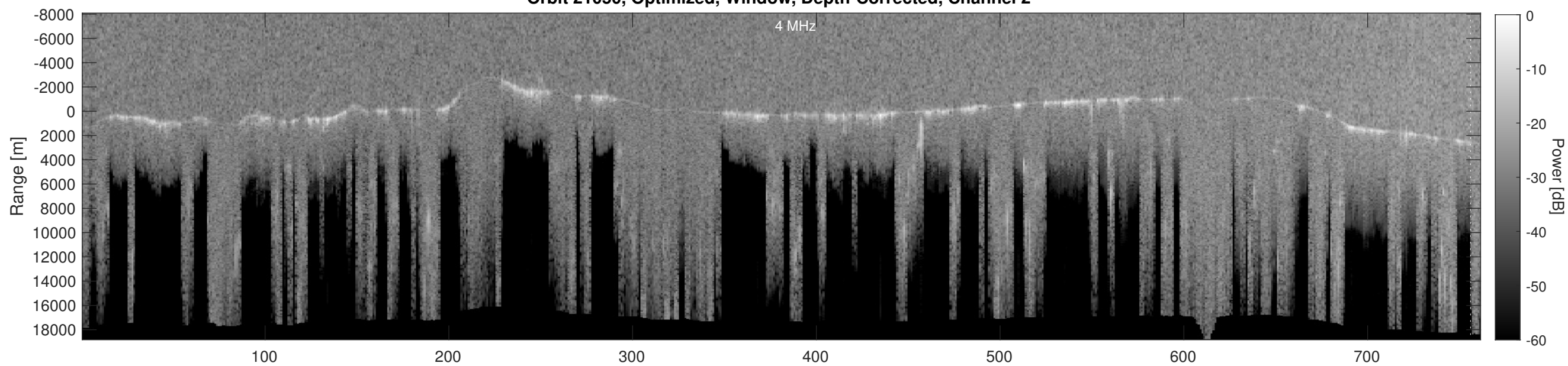
Orbit 21050, Depth-Corrected Cluttergram
