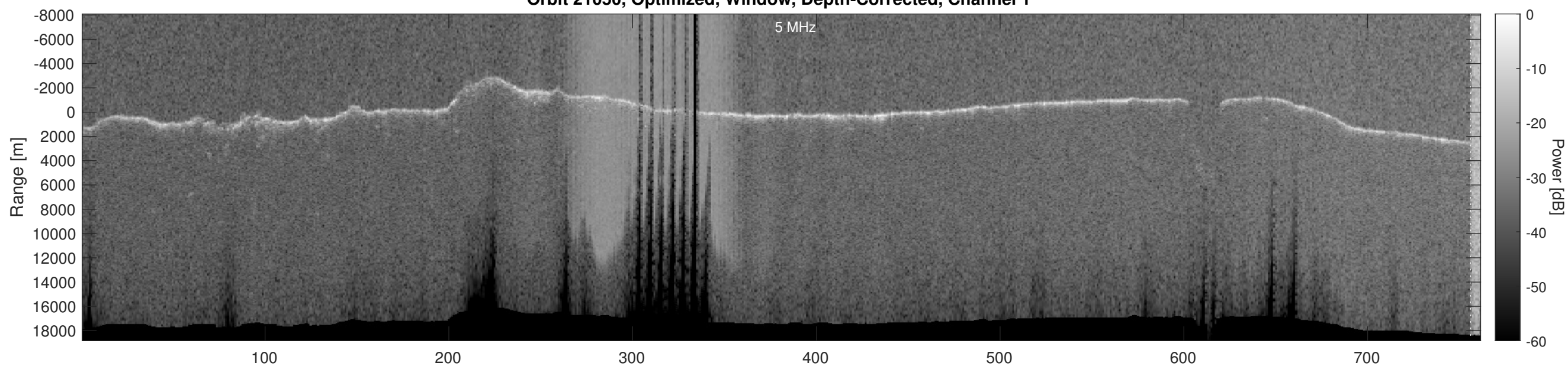
Orbit 21050, Optimized, Window, Depth-Corrected, Channel 2
