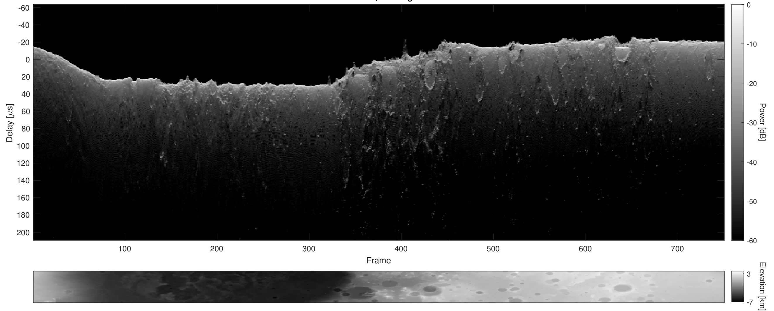
Orbit 21052, Cluttergram
