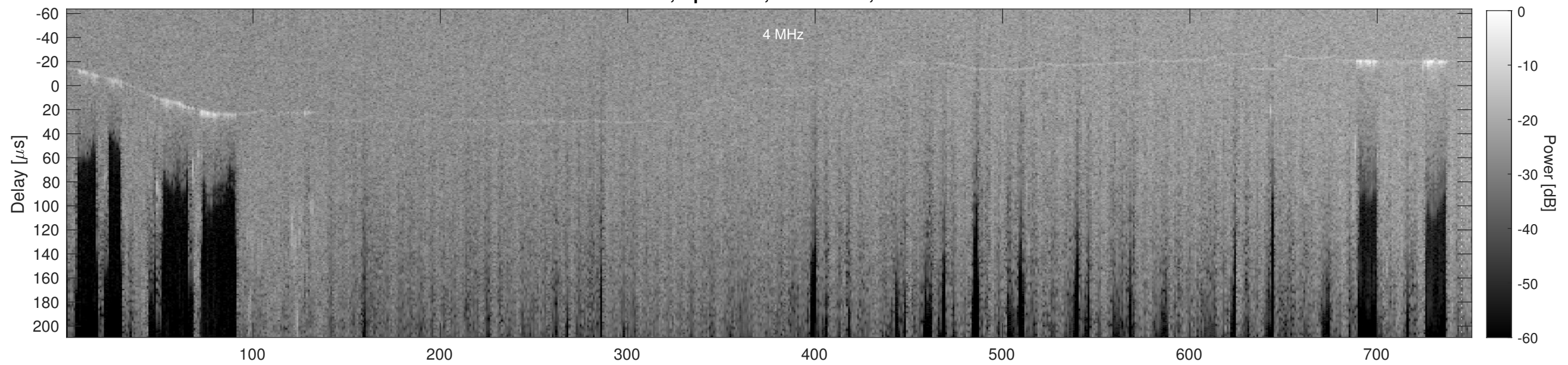
Orbit 21052, Cluttergram
