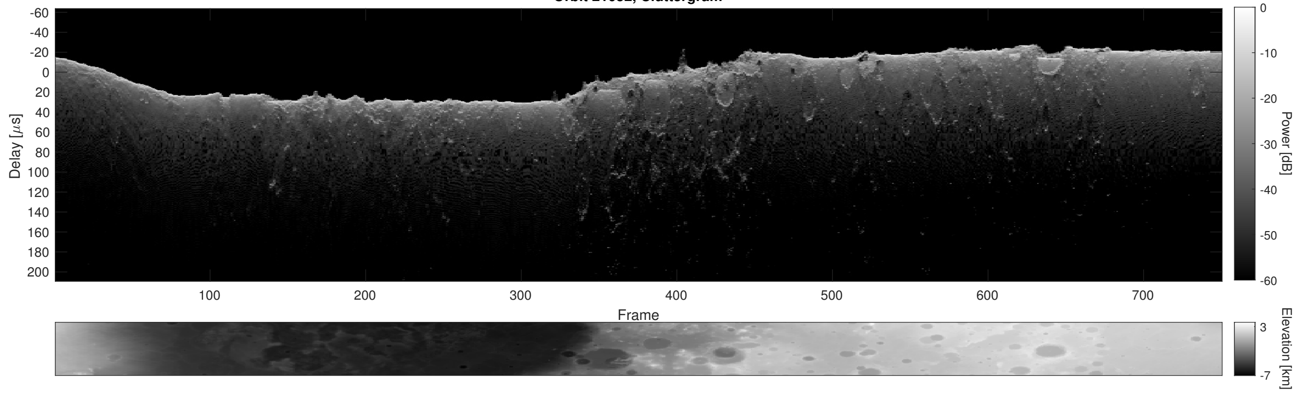
Orbit 21052, Cluttergram
