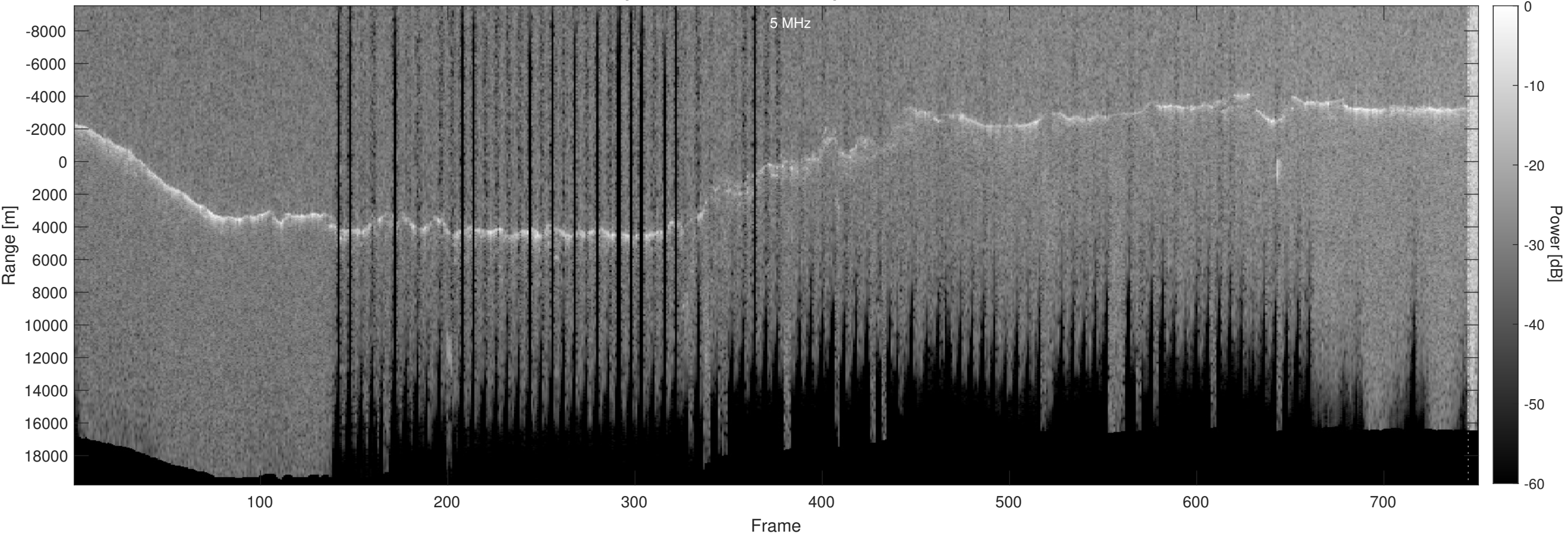
Orbit 21052, Optimized, No Window, Depth-Corrected, Channel 2
