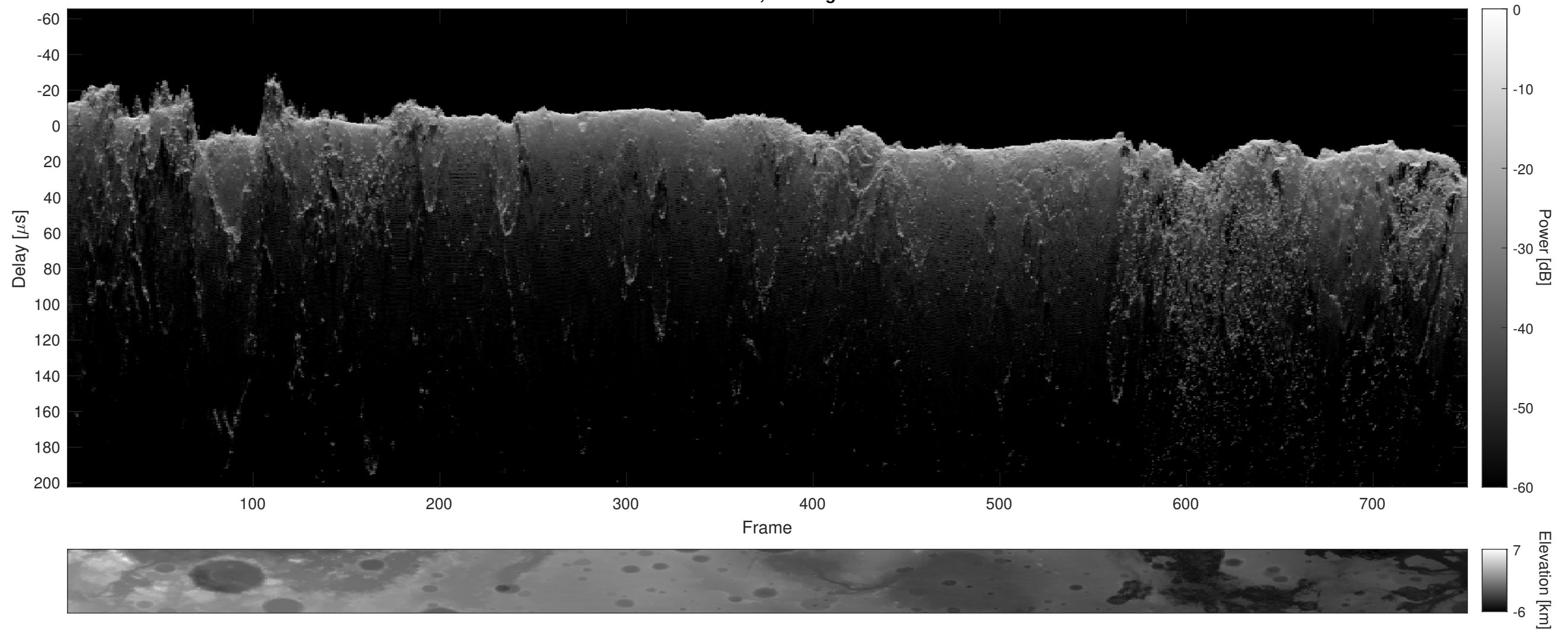
Orbit 21053, Cluttergram
