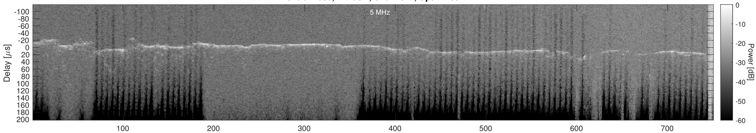
Orbit 21053, Cluttergram
