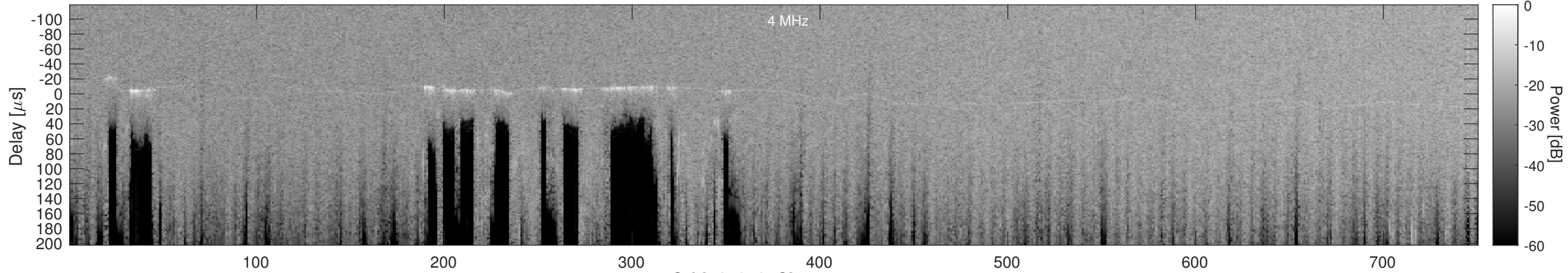
Orbit 21053, Cluttergram
