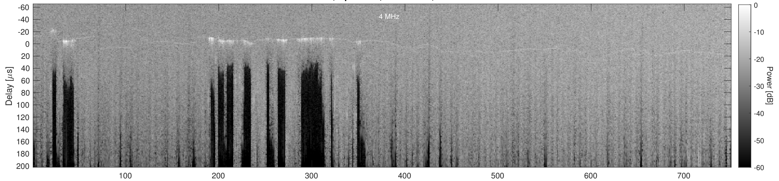
Orbit 21053, Cluttergram
