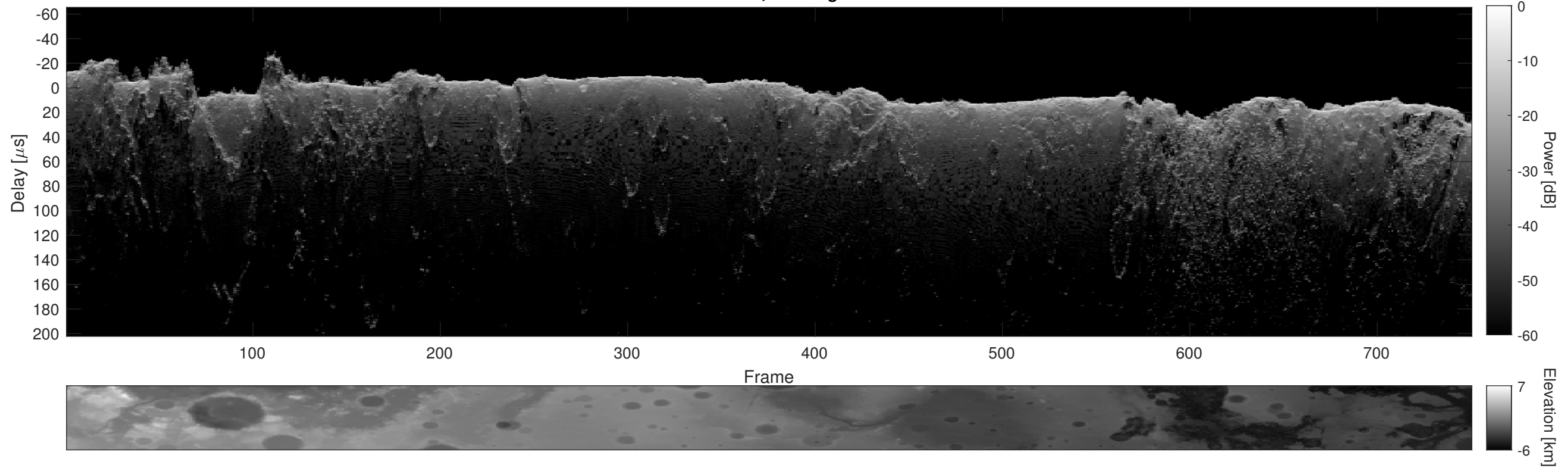
Orbit 21053, Cluttergram
