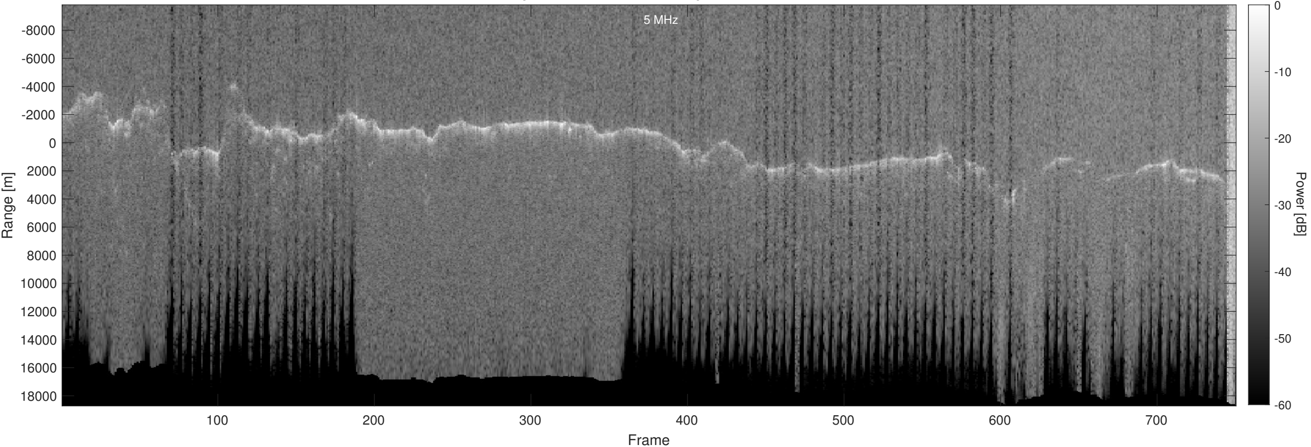
Orbit 21053, Optimized, No Window, Depth-Corrected, Channel 2
