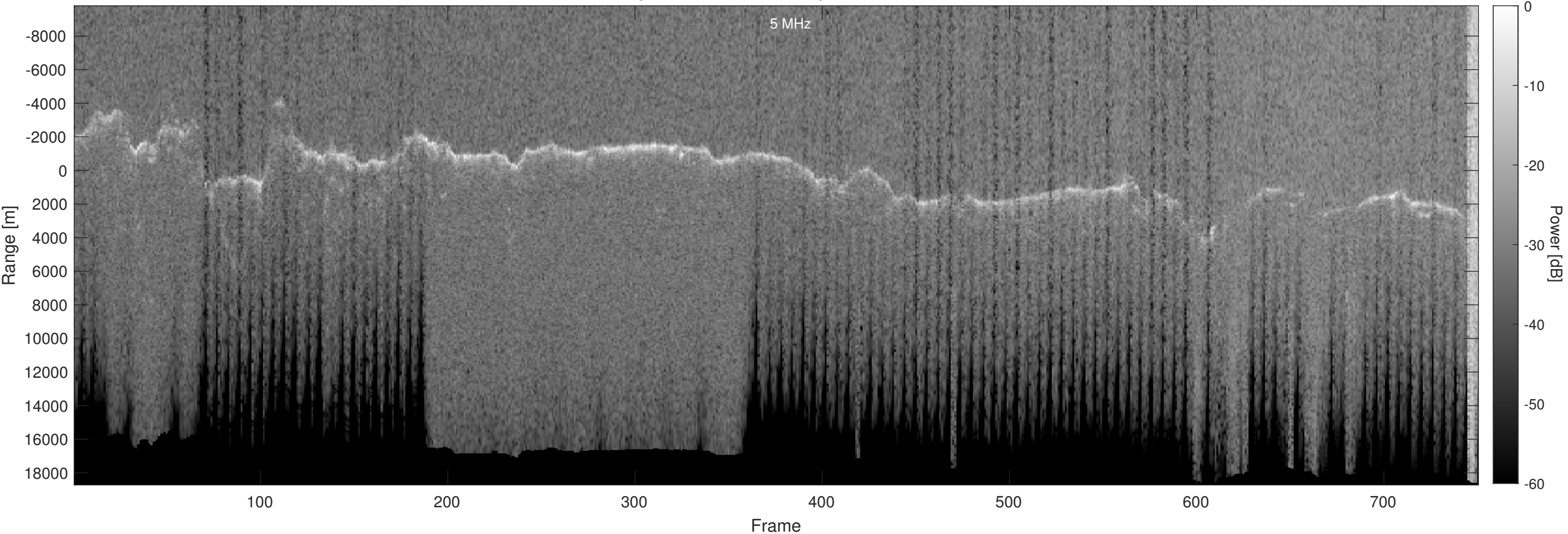
Orbit 21053, Optimized, Window, Depth-Corrected, Channel 2
