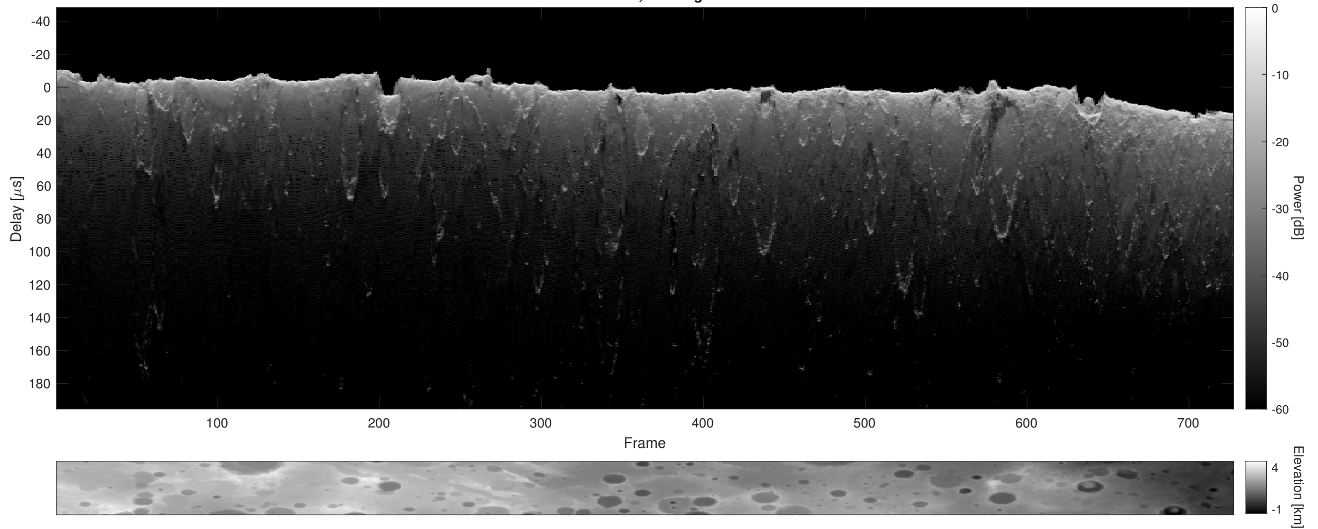
Orbit 21056, Cluttergram
