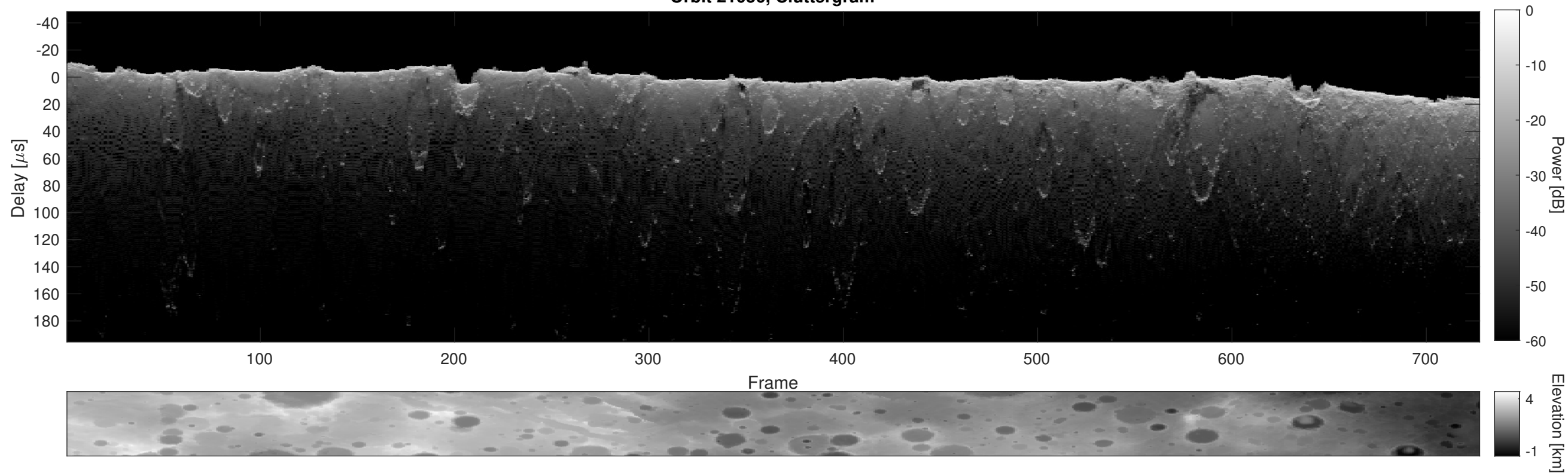
Orbit 21056, Cluttergram
