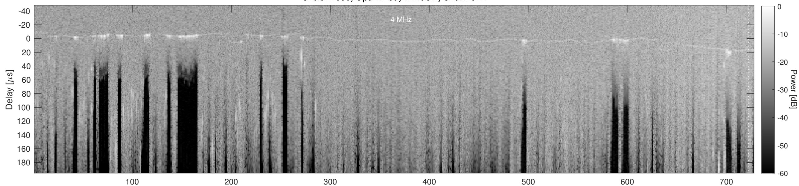
Orbit 21056, Cluttergram
