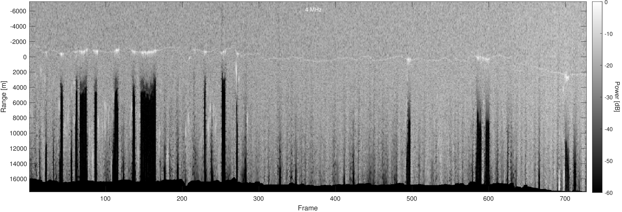
Orbit 21056, Optimized, Window, Depth-Corrected, Channel 2
