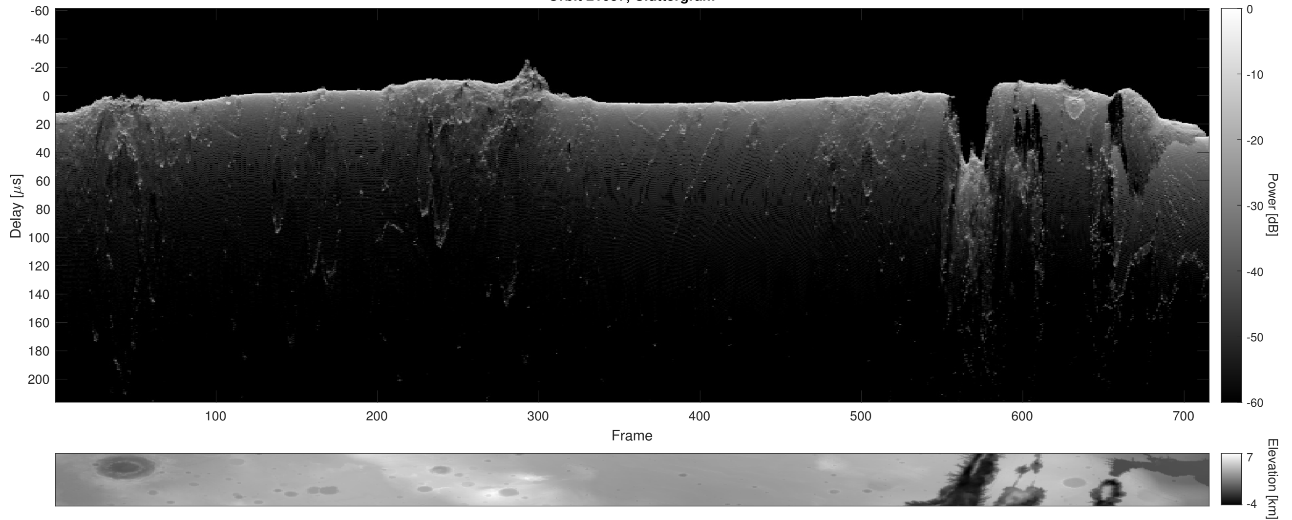
Orbit 21057, Cluttergram
