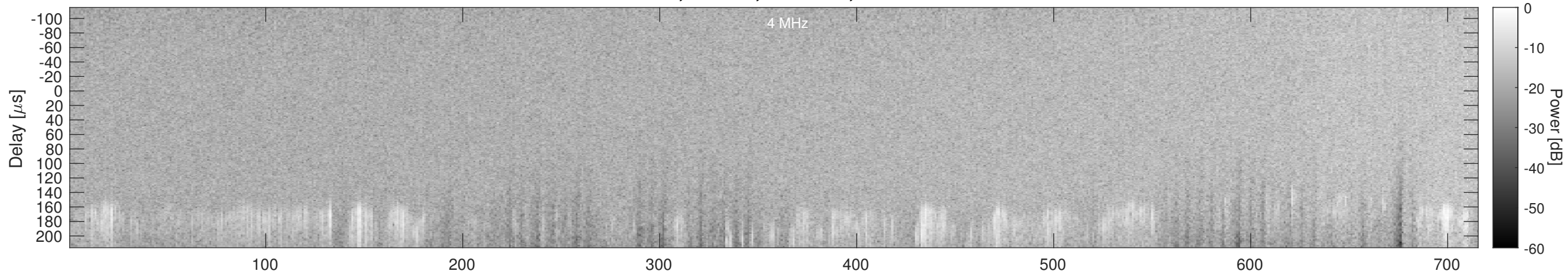
Orbit 21057, Window, Channel 2, Chapman
