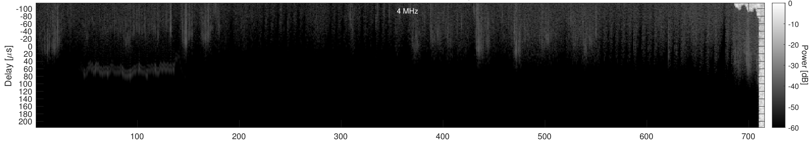
Orbit 21057, Window, Channel 2, Optimized
