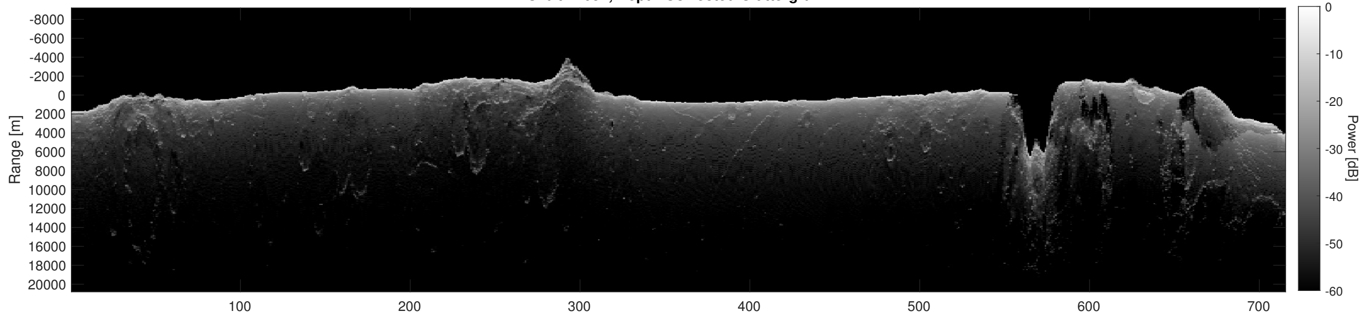
Orbit 21057, Depth-Corrected Cluttergram
