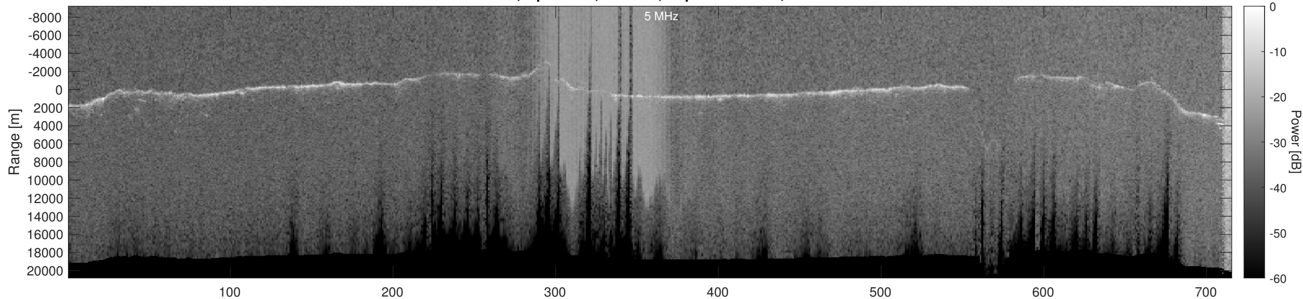
Orbit 21057, Optimized, Window, Depth-Corrected, Channel 2
