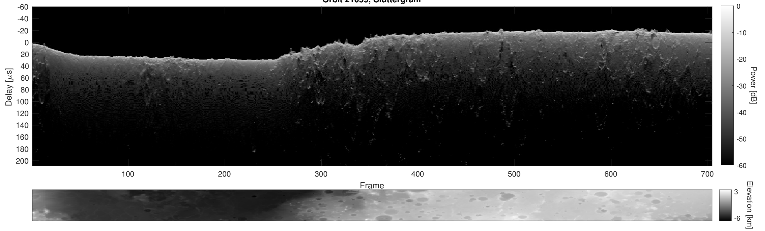
Orbit 21059, Cluttergram
