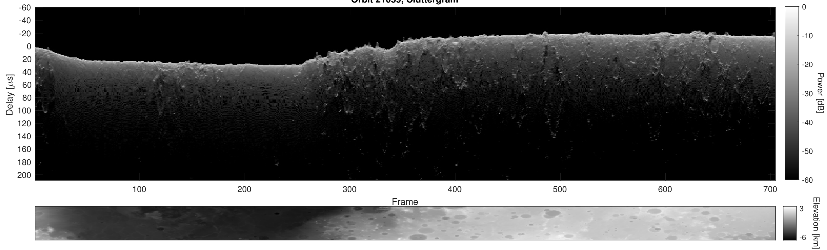
Orbit 21059, Cluttergram
