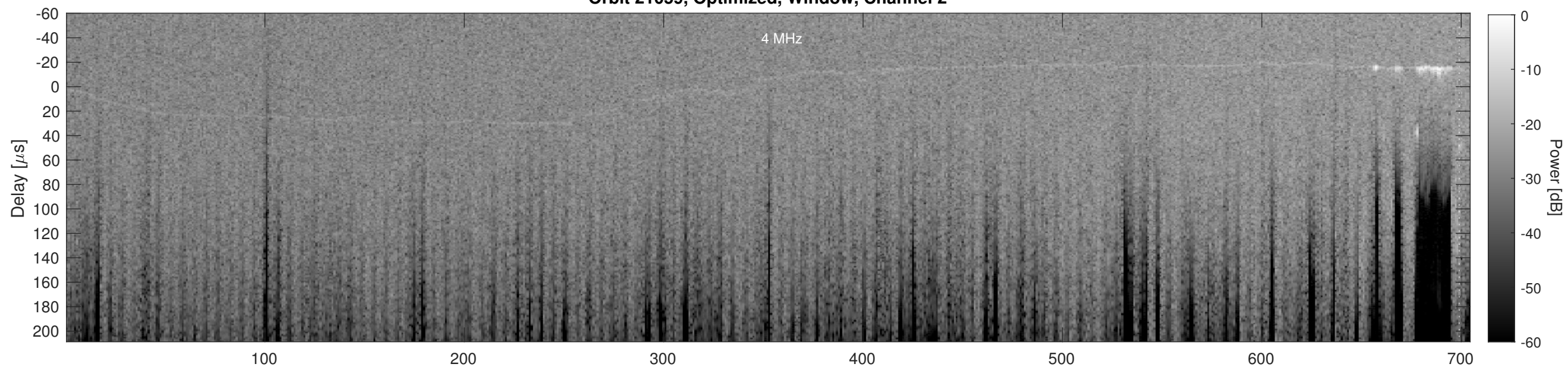
Orbit 21059, Cluttergram
