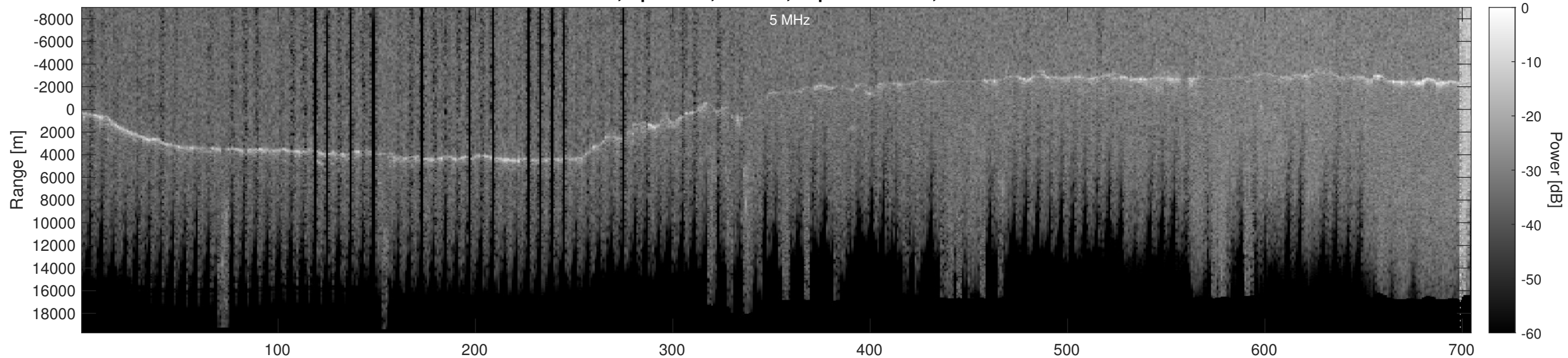
Orbit 21059, Optimized, Window, Depth-Corrected, Channel 2
