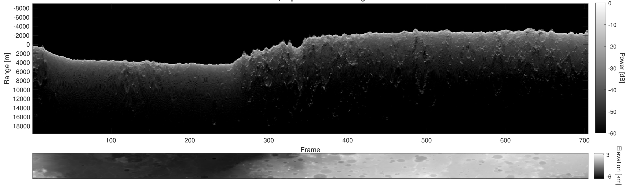
Orbit 21059, Depth-Corrected Cluttergram
