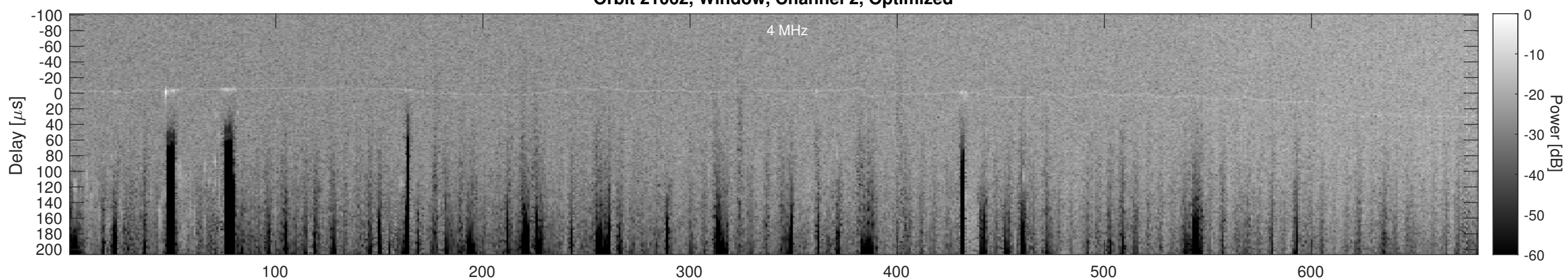
Orbit 21062, Cluttergram
