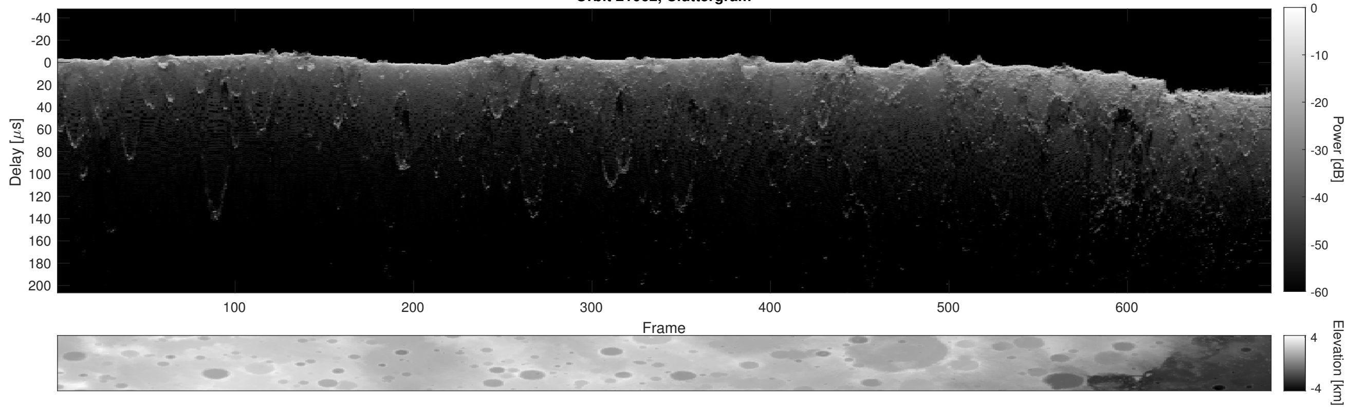
Orbit 21062, Cluttergram
