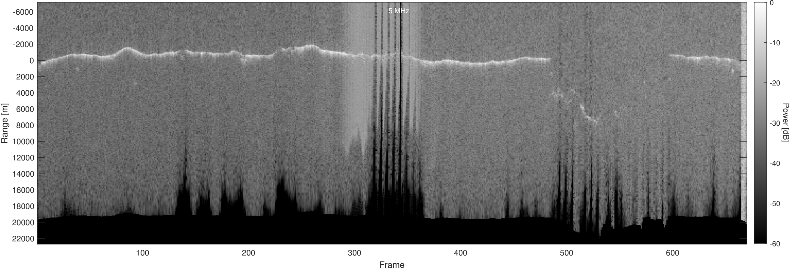
Orbit 21064, Optimized, No Window, Depth-Corrected, Channel 2
