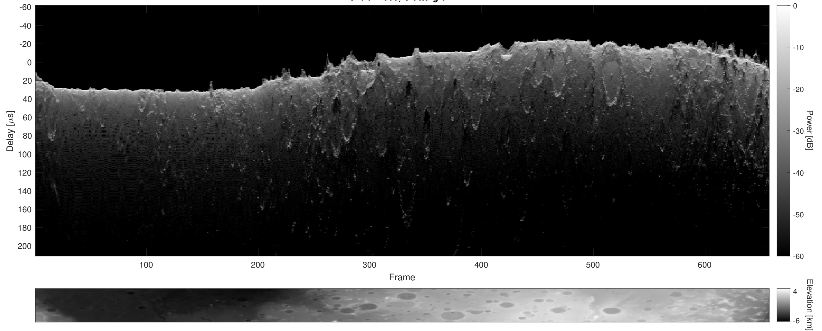
Orbit 21066, Cluttergram
