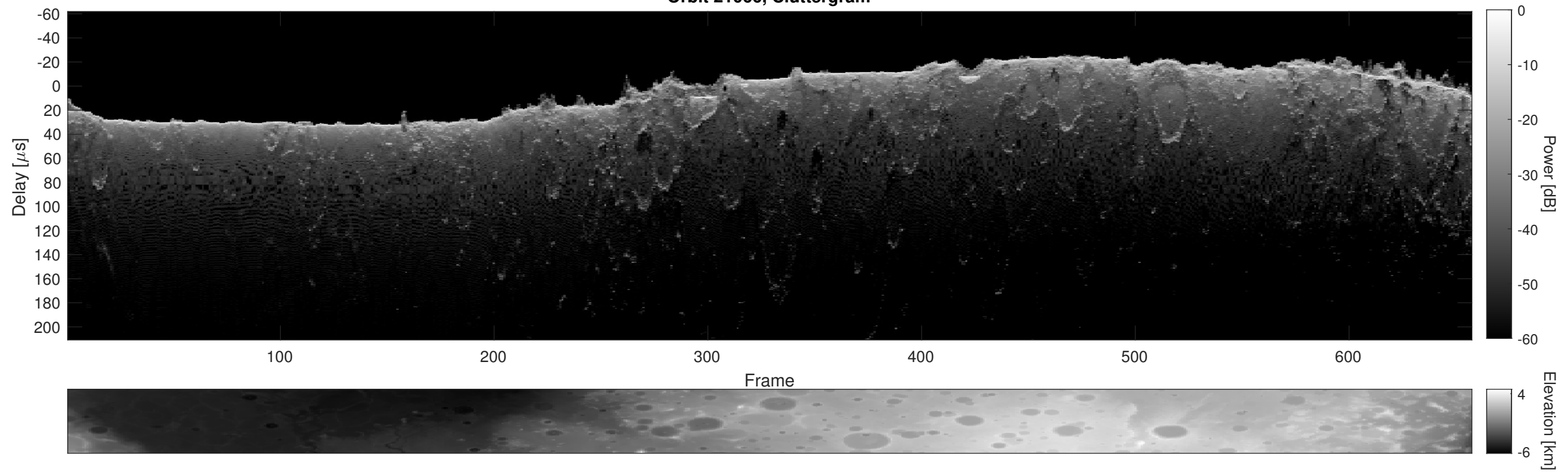
Orbit 21066, Cluttergram
