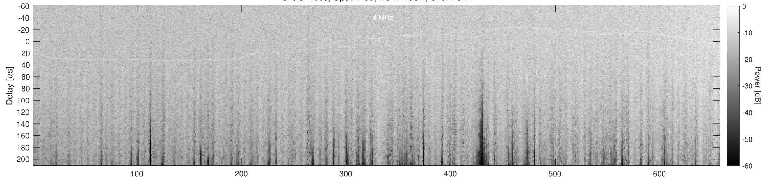
Orbit 21066, Cluttergram
