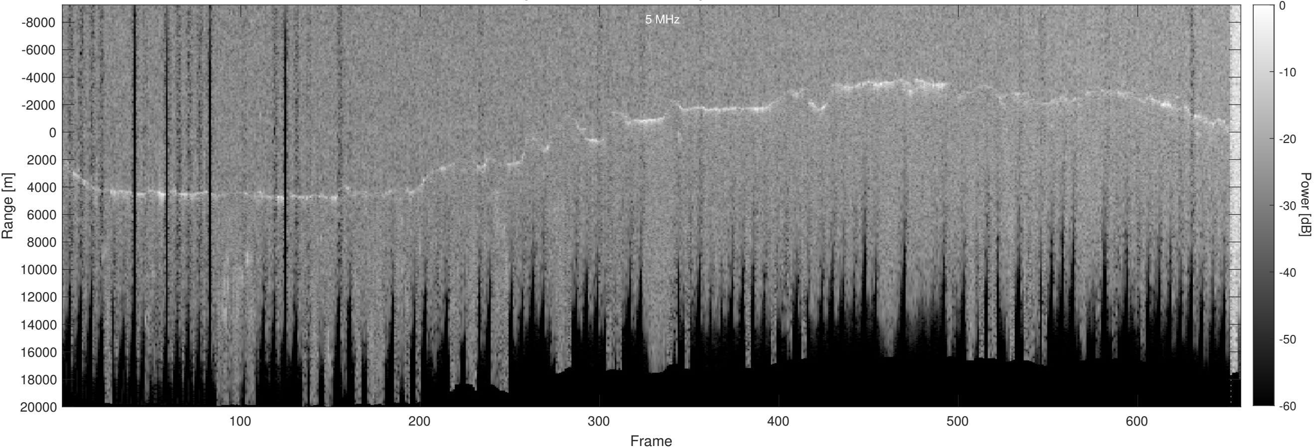
Orbit 21066, Optimized, No Window, Depth-Corrected, Channel 2
