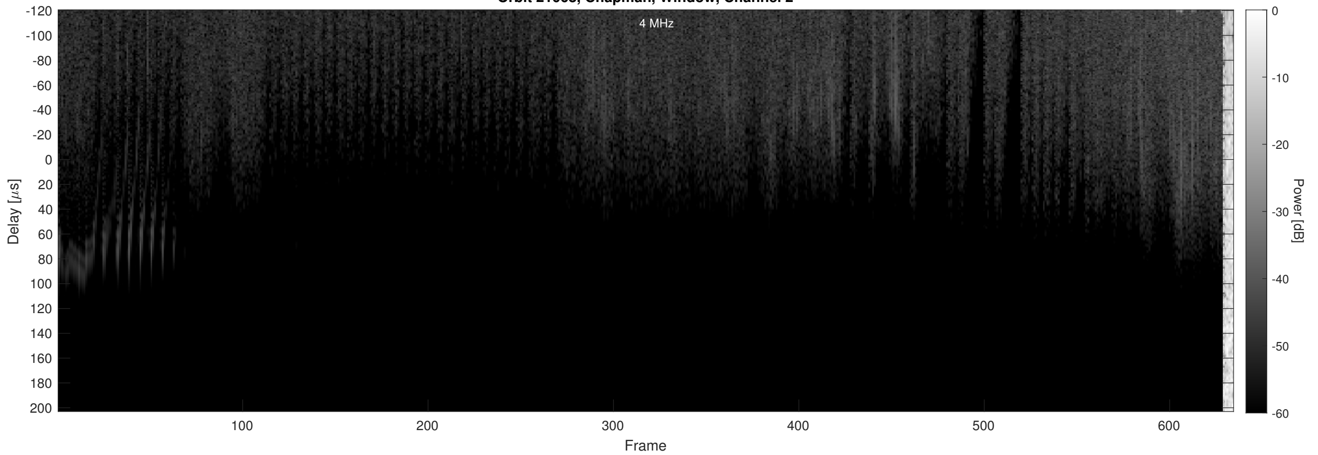
Orbit 21068, Chapman, Window, Channel 2
