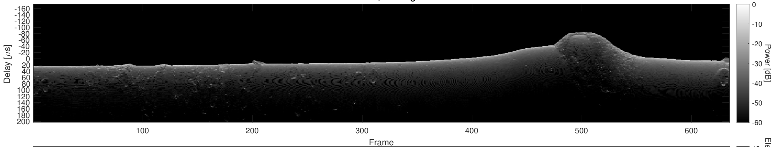
Orbit 21068, Cluttergram
