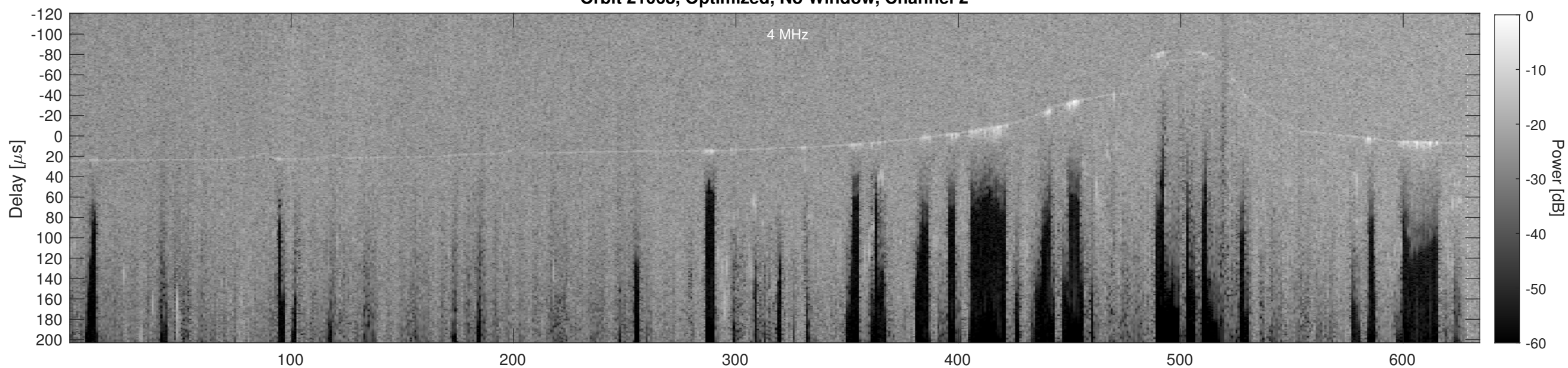
Orbit 21068, Cluttergram
