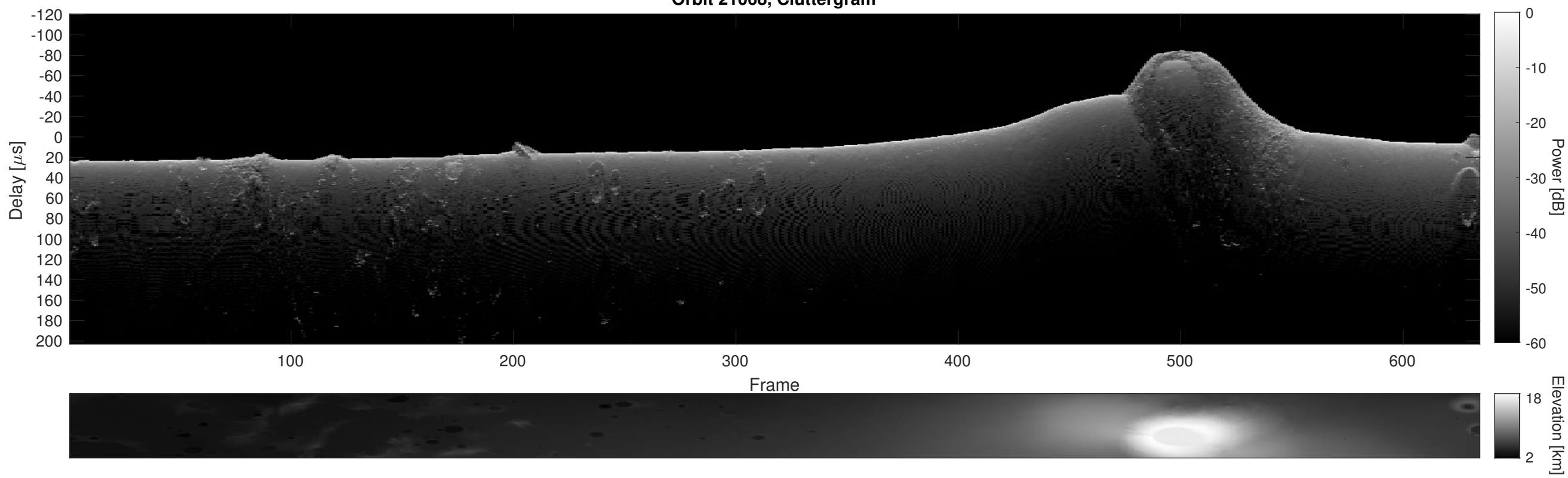
Orbit 21068, Cluttergram
