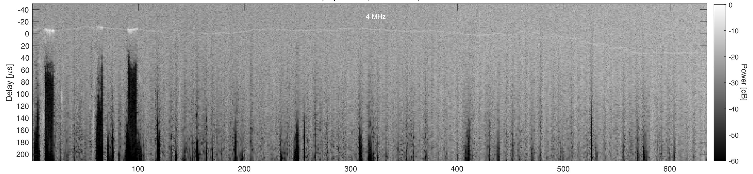
Orbit 21069, Cluttergram
