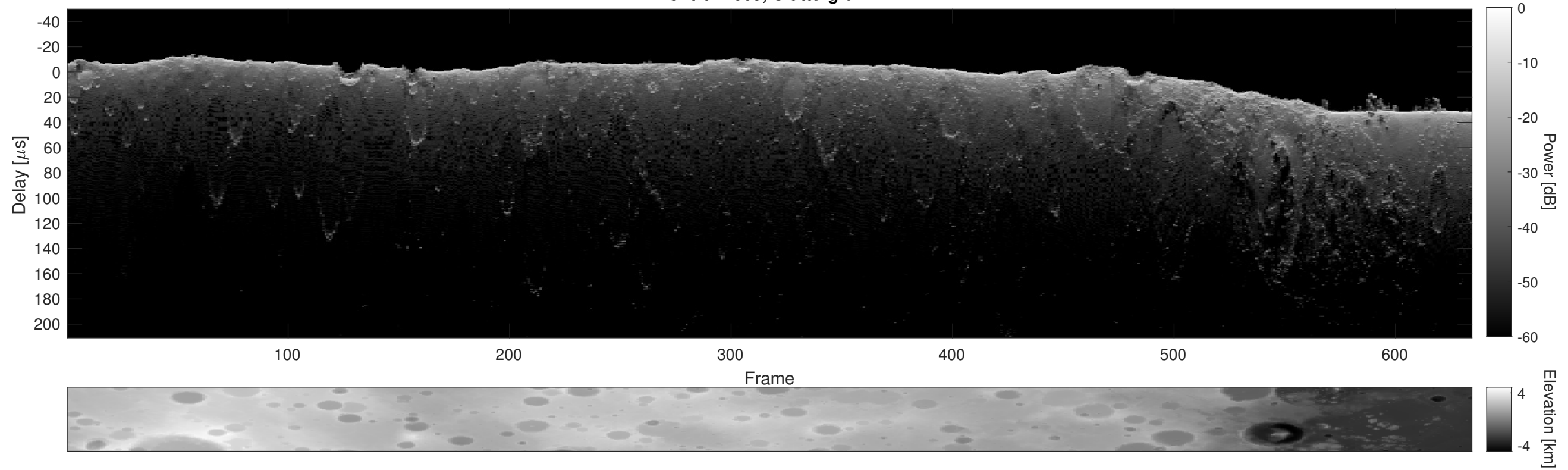
Orbit 21069, Cluttergram
