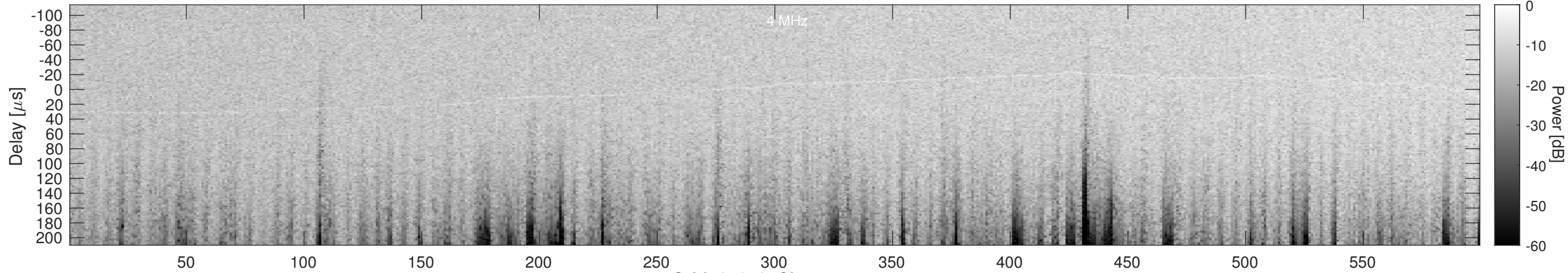
Orbit 21073, Cluttergram
