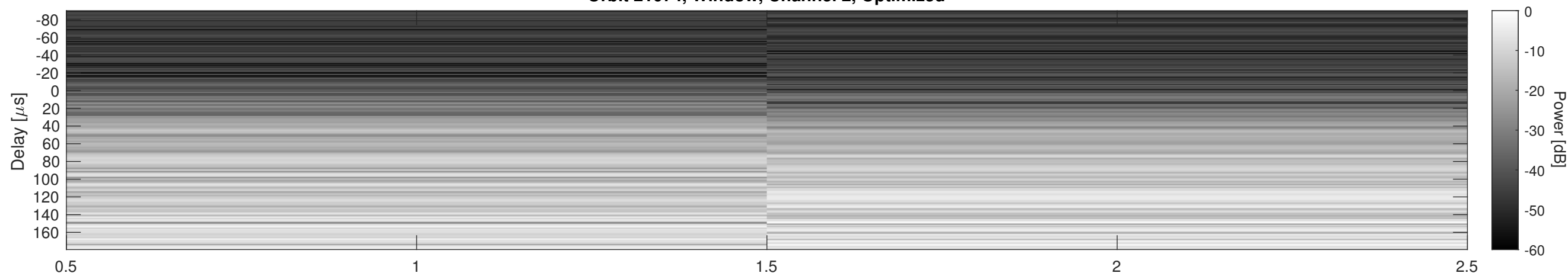
Orbit 21074, Cluttergram
