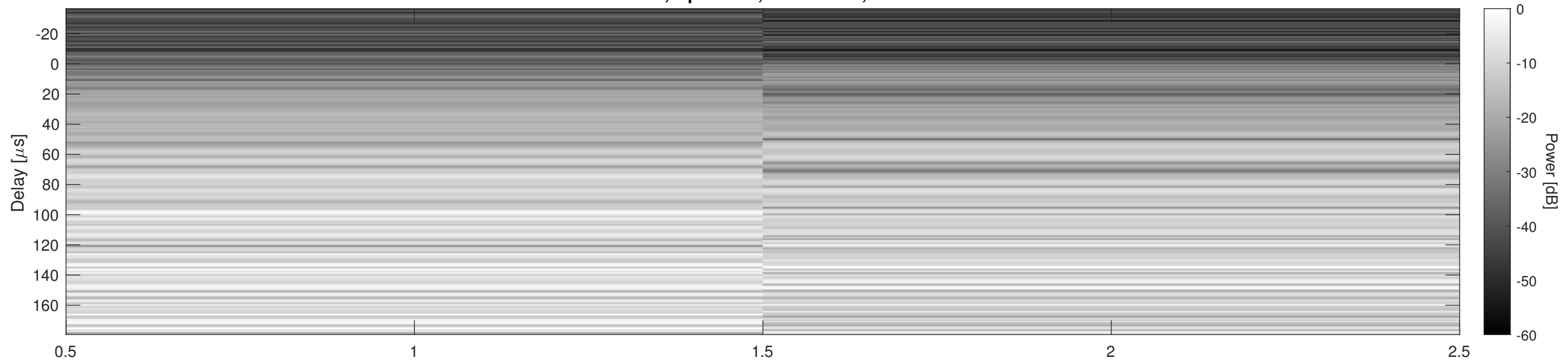
Orbit 21074, Optimized, No Window, Channel 2
