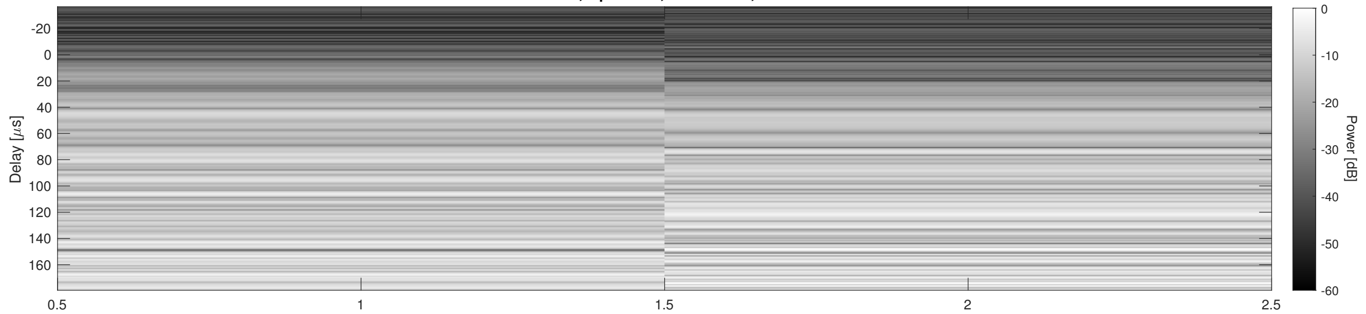
Orbit 21074, Cluttergram
