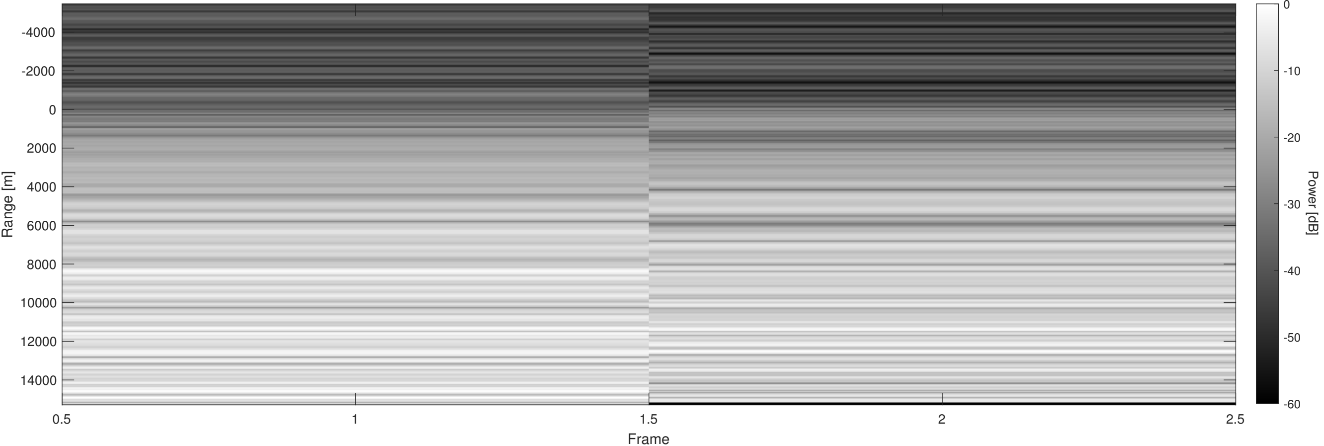
Orbit 21074, Optimized, No Window, Depth-Corrected, Channel 2
