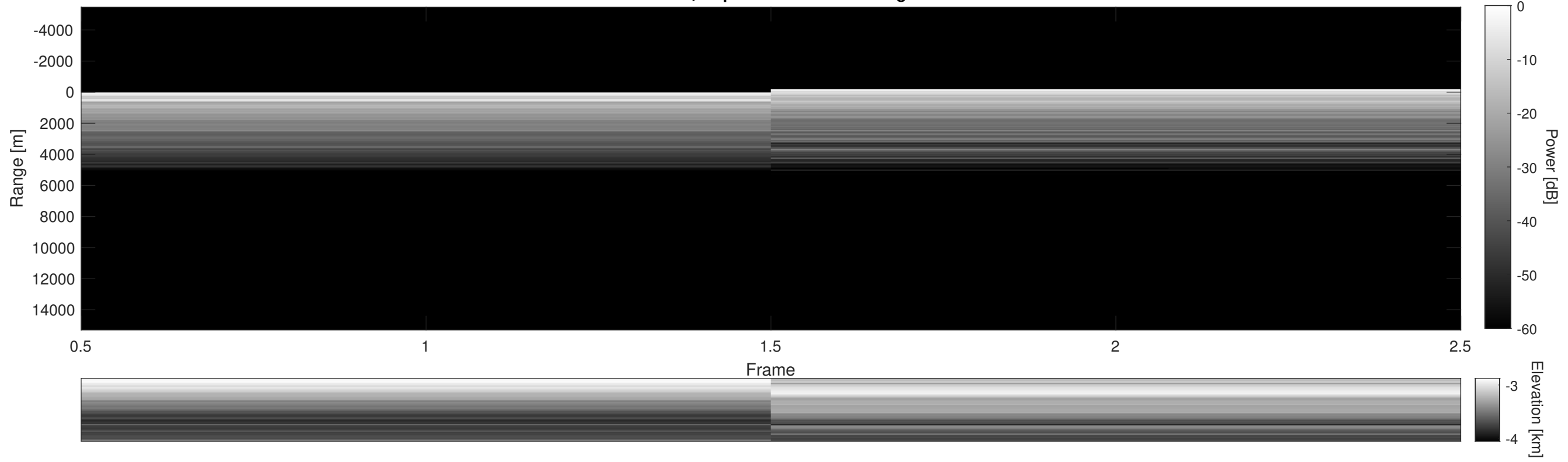
Orbit 21074, Depth-Corrected Cluttergram
