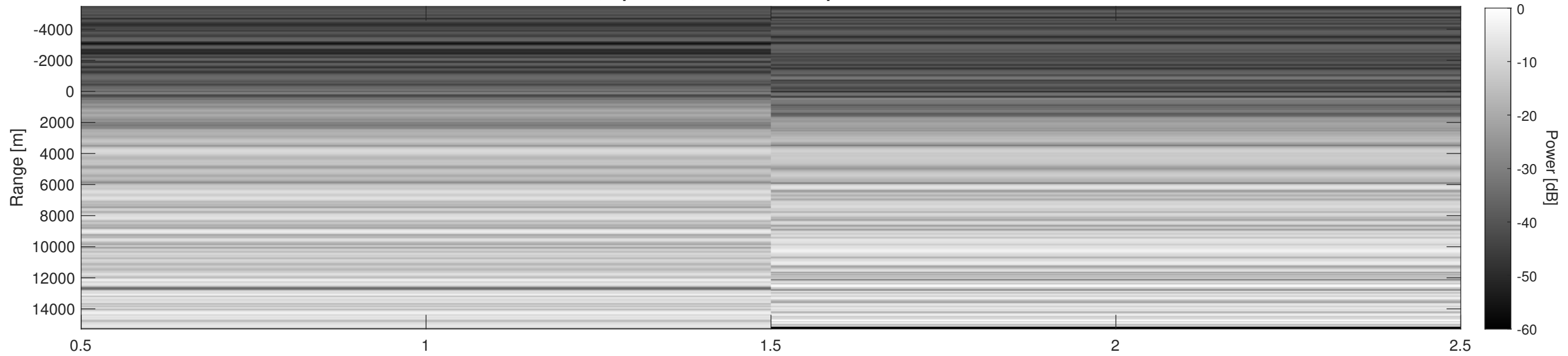
Orbit 21074, Depth-Corrected Cluttergram
